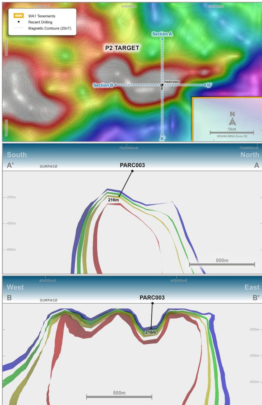
Figures 3-5: Top - Plan View, Middle – Cross-section, Bottom - Long-section Schematics of gravity anomaly images (residual gravity with 2.68-2.72g/cc density shells)
