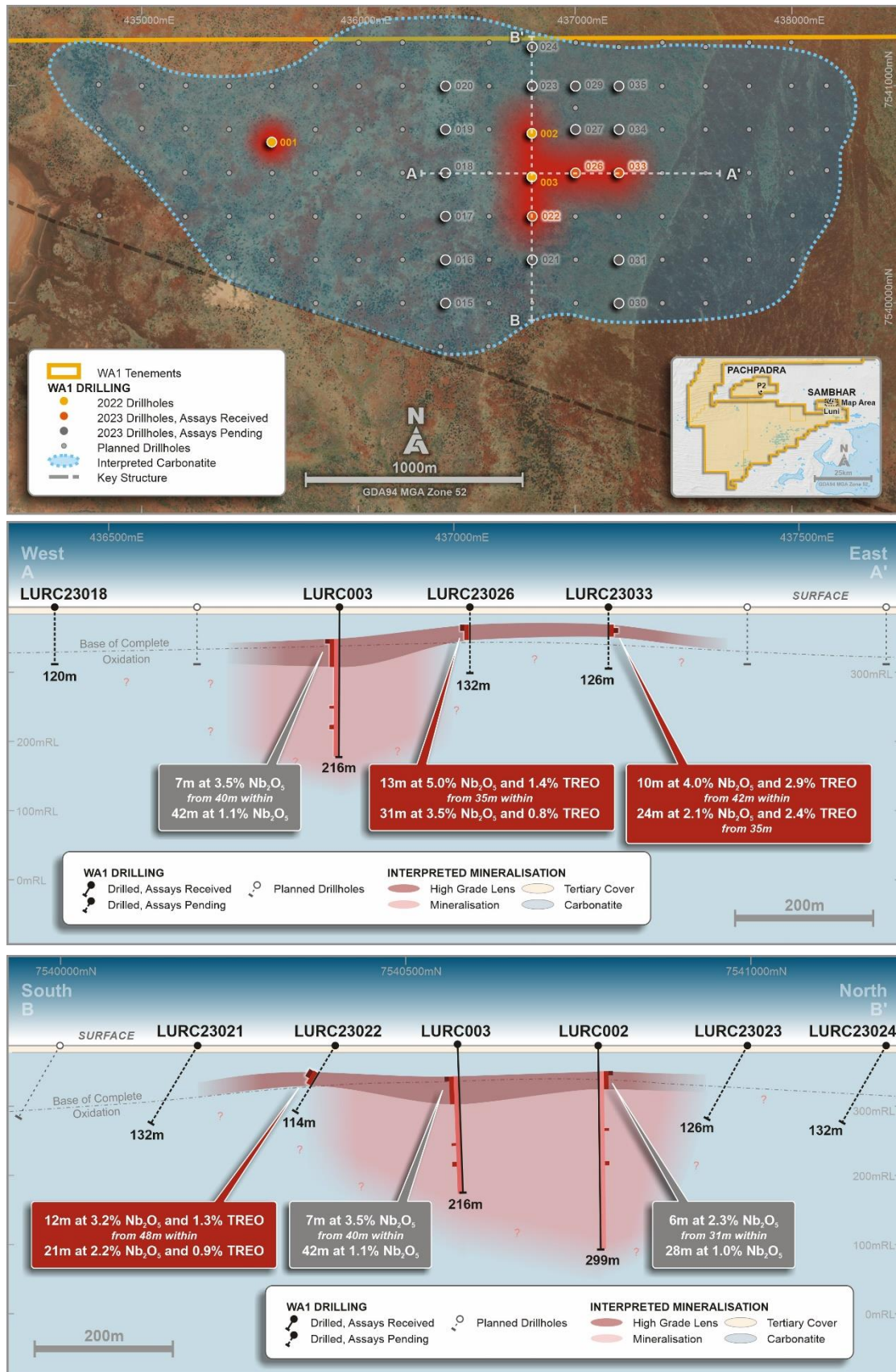
Figures 1-3: Top – Luni carbonatite plan view and drill collar locations, Middle – Simplified long-section looking north, Bottom – Simplified cross-section looking west
