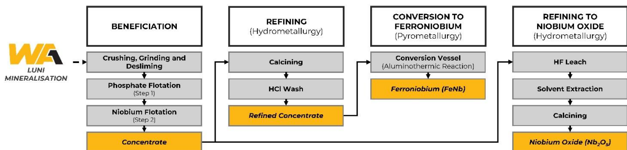
Figure 4: Simplified process flowsheet to produce proof-of-concept ferroniobium and niobium oxide
