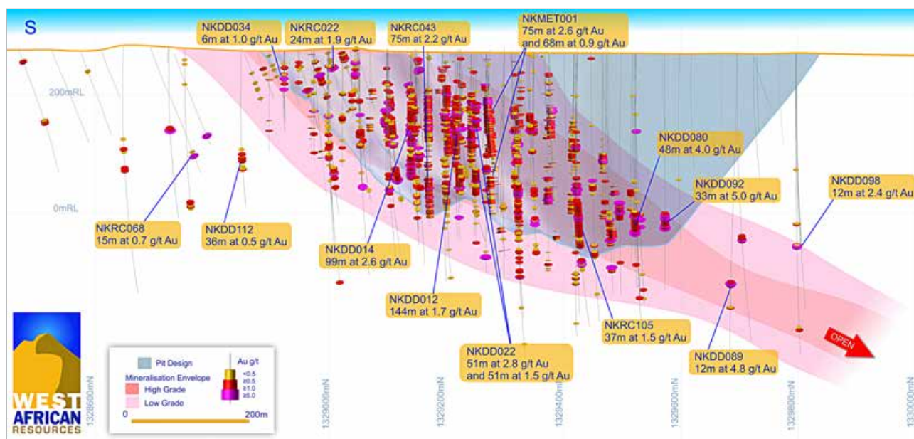
Figure 9 – Toega long section
