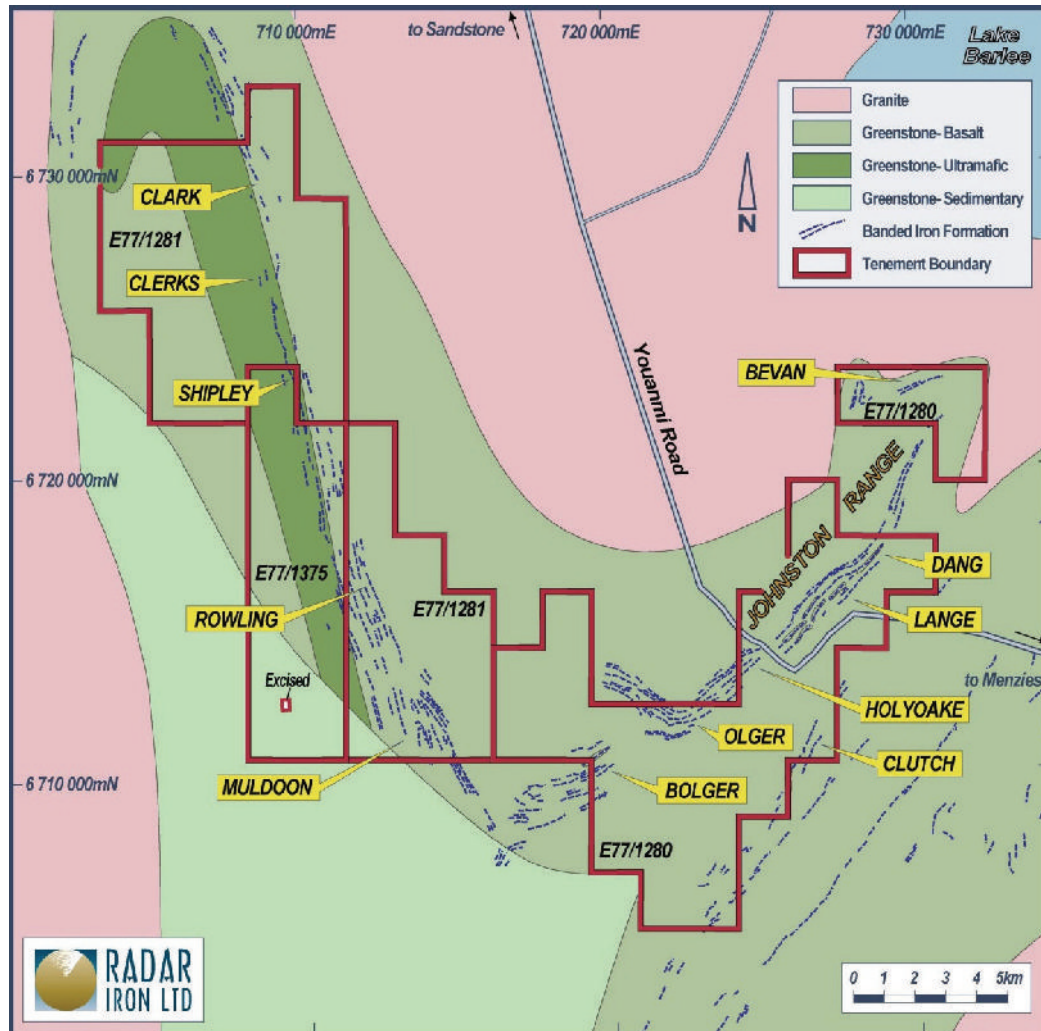
Figure 9. Johnston Range/Copper Bore Project - Prospect Locations
