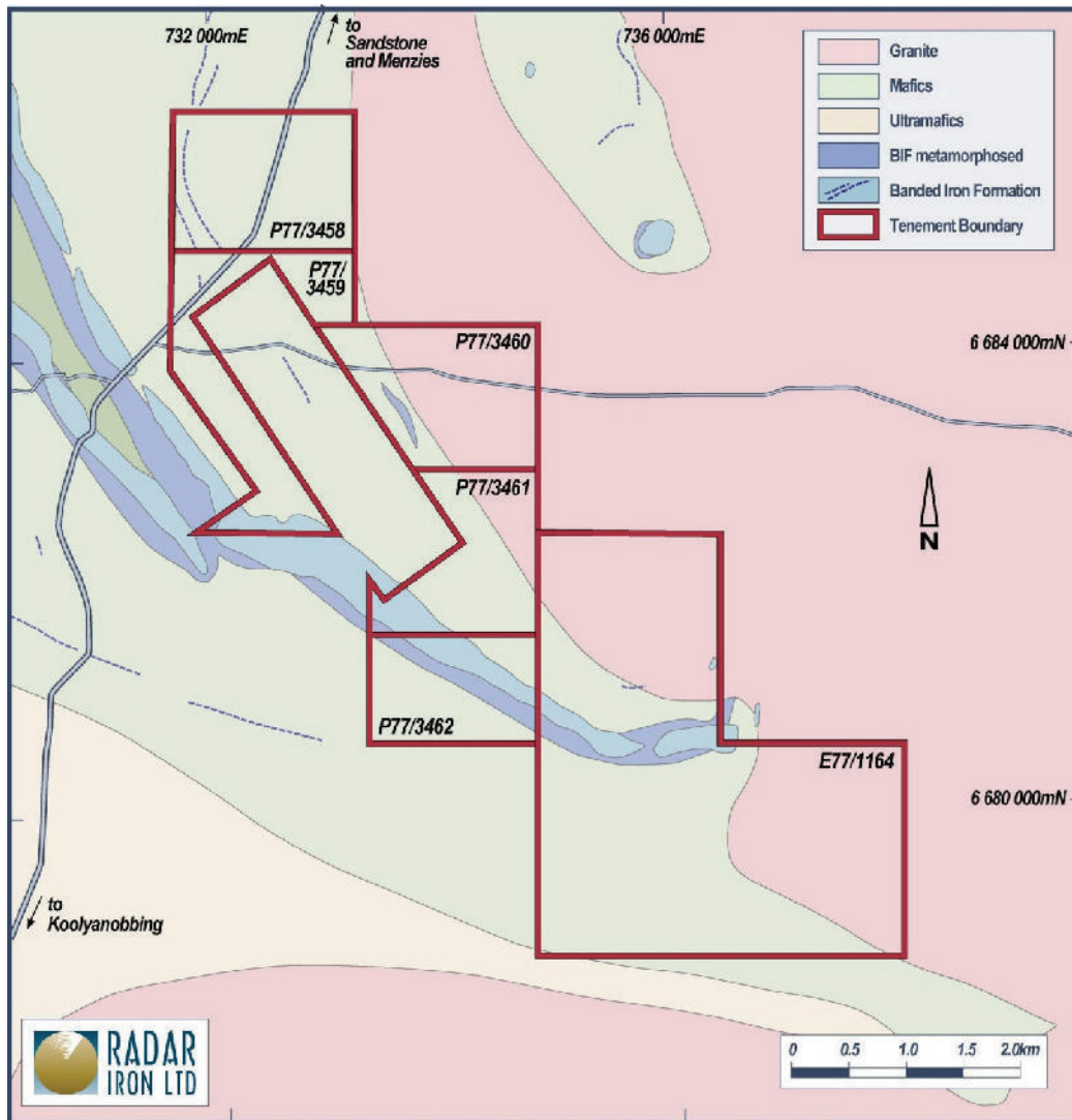
Figure 12. Die Hardy Project Northern Tenements – Simplified Geology
