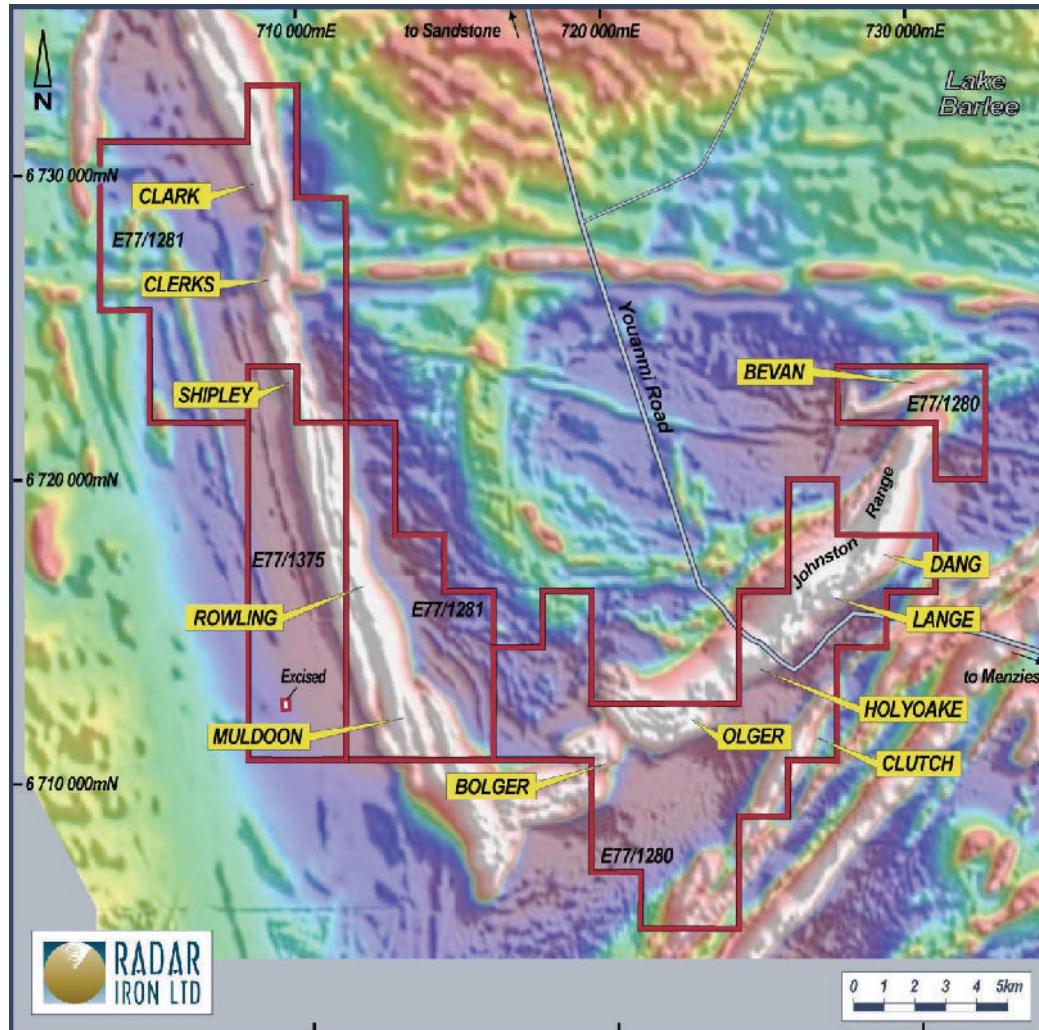
Figure 10. Johnston Range/Copper Bore Imaged Aeromagnetic Data
