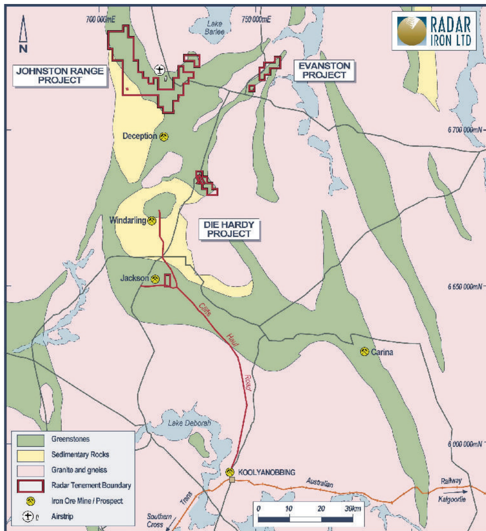
Figure 3 – Regional Geology
