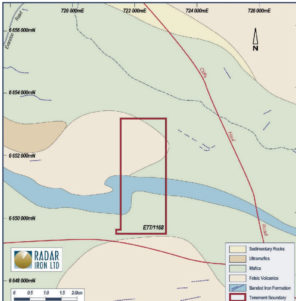
Figure 13. Die Hardy Project Southern Tenement – Simplified Geology
