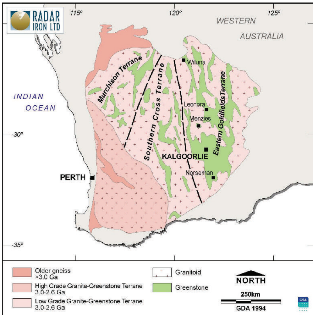
Figure 4. Yilgarn Craton and Major Greenstone Belts
