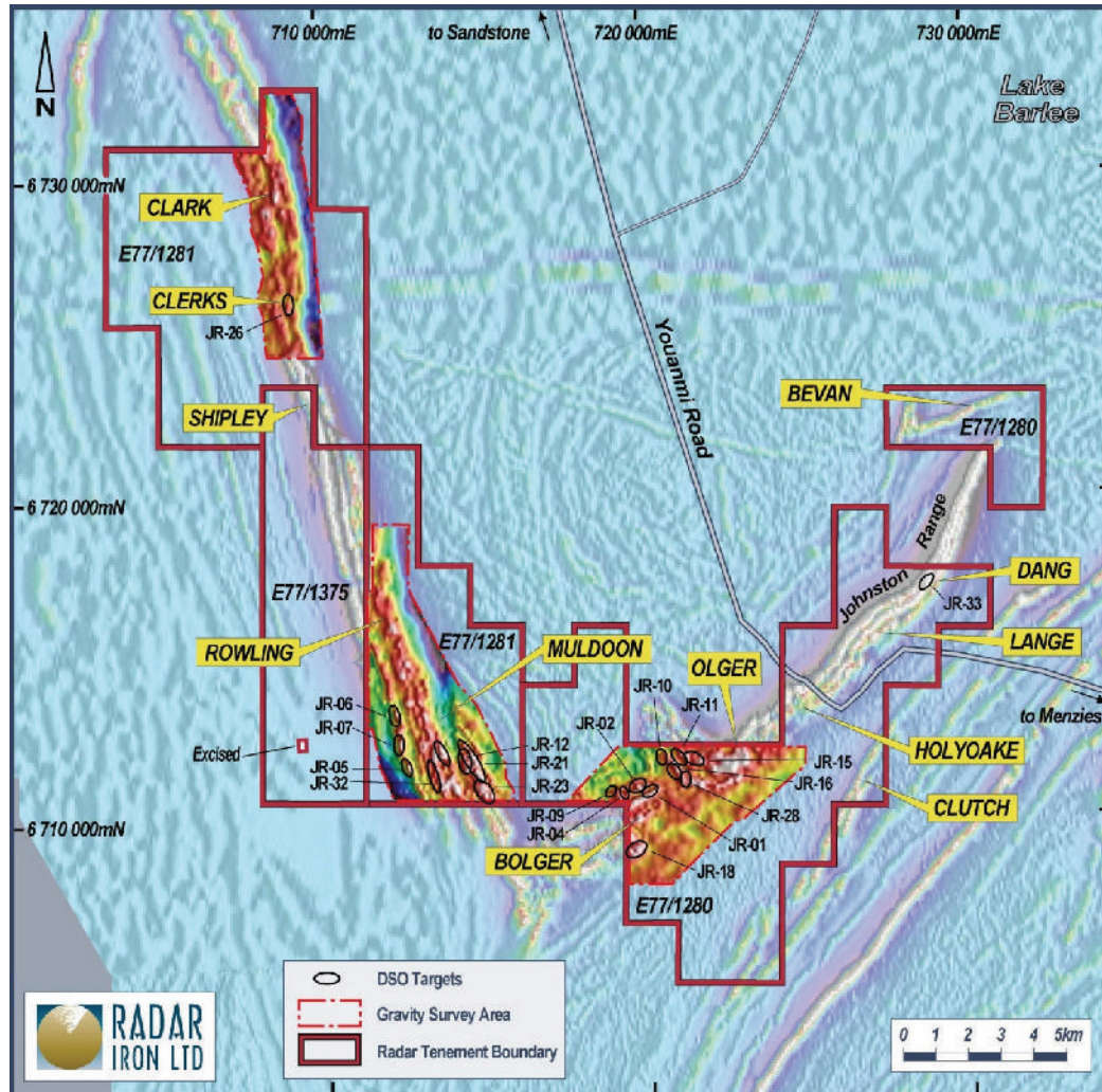
Figure 11. Johnston Range/Copper Bore Goethite-Hematite Targets and Extent of Gravity Overlay on Aeromagnetic Image.
