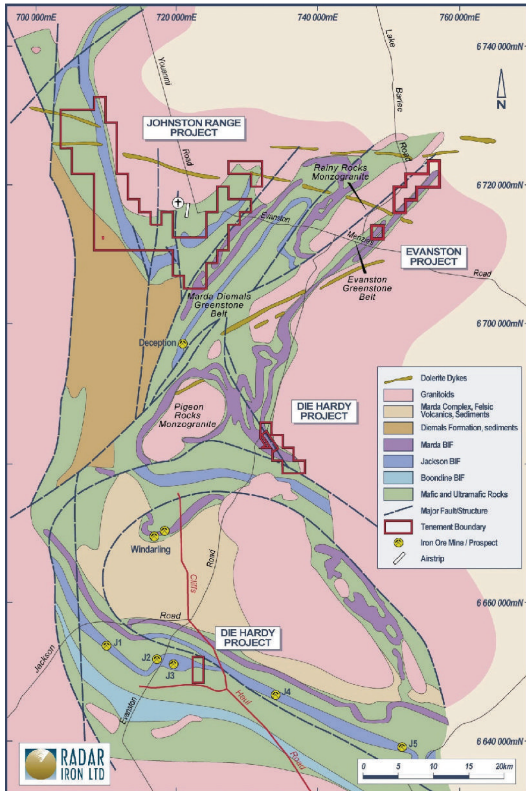
Figure 5. Simplified Geology Marda-Diemals and Evanston Greenstone Belts
