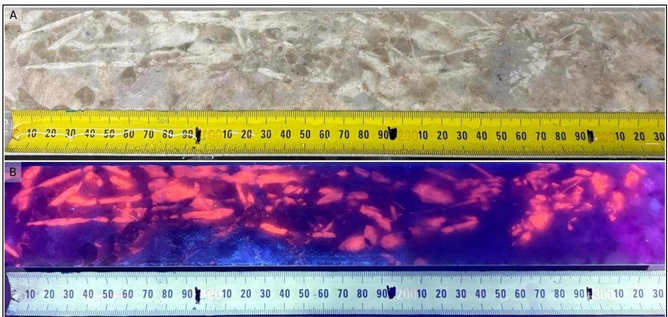
Figure 1: Top (A): Core from BCDD004 from 76.54 to 76.87m in natural light. Elongate white crystals are interpreted as spodumene. Bottom (B) The same core exposed to UV light confirming the elongate crystals fluoresce at a wavelength typical of spodumene (orange). Logged mineral abundance estimations provided (Table 4).
