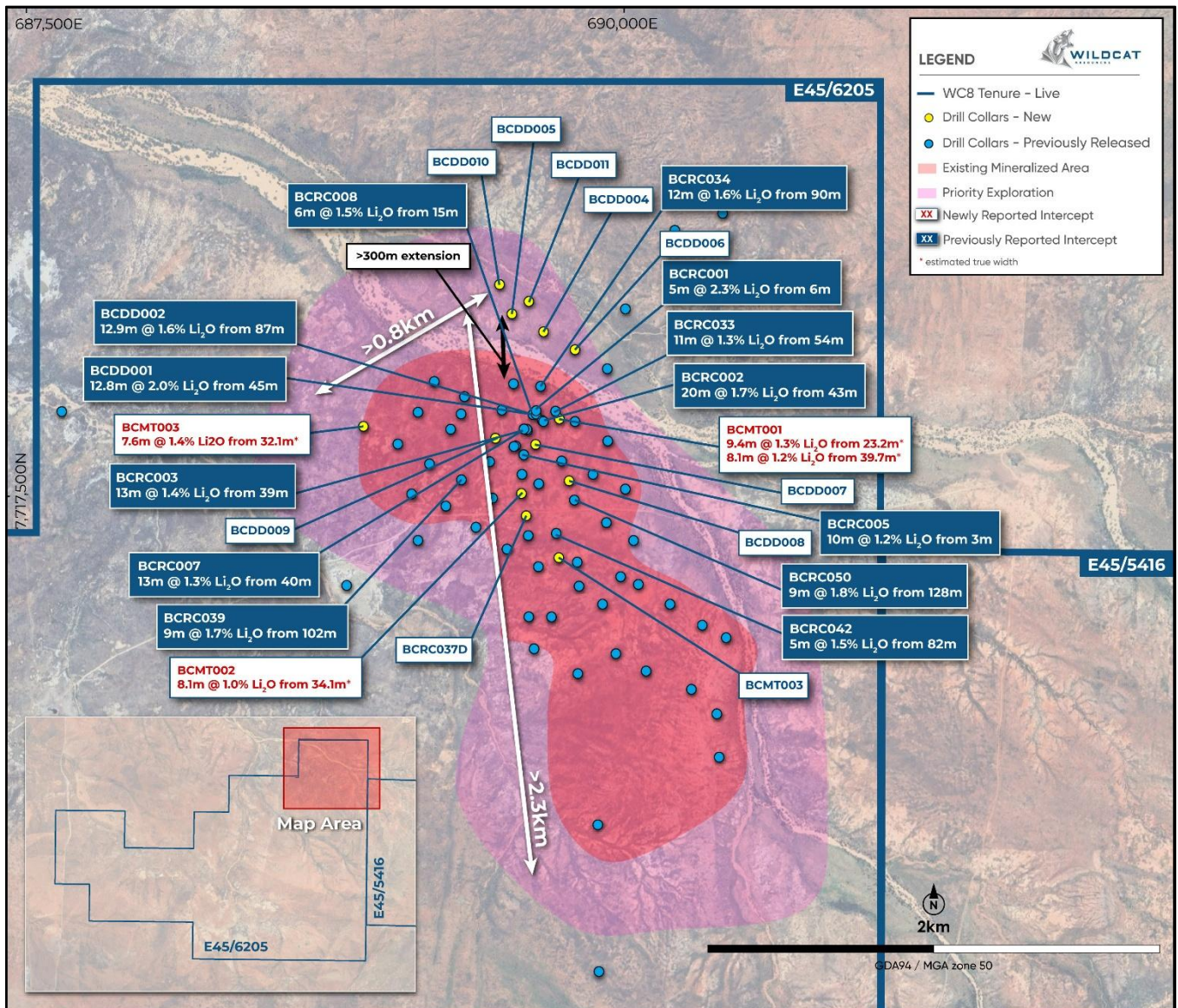
Figure 2: Plan of Bolt Cutter Central showing existing lithium intercepts (rounded to 1 decimal point) and locations of exploration and metallurgical drillholes (BCMT001-003). Mineralisation (>0.5% Li 2 O) in the pegmatite swarms remain open in most directions.
