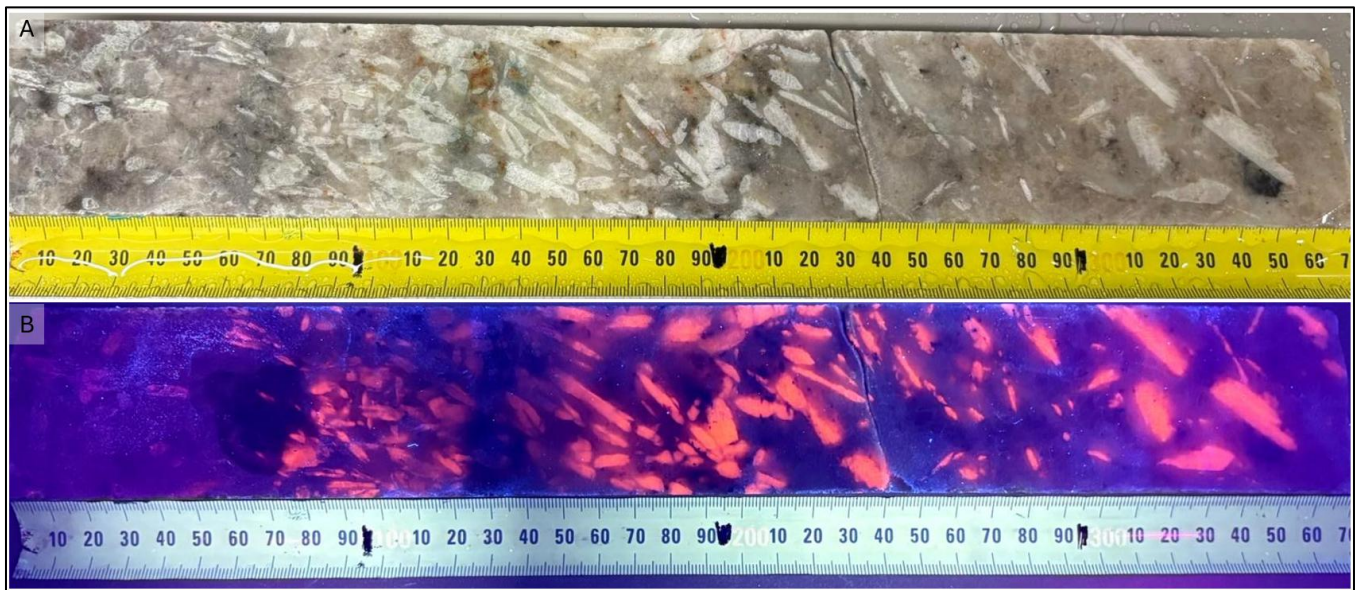
Figure 3: Top (A): Core from BCDD006 from 132.94 to 133.3m in natural light. Elongate white crystals are interpreted as spodumene. Bottom (B) The same core exposed to UV light confirming the elongate crystals fluoresce at a wavelength typical of spodumene (orange). Logged mineral abundance estimations provided (Table 4).
