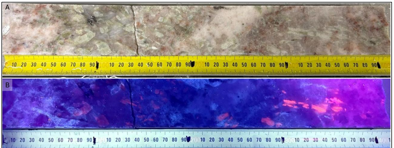
Figure 4: Top (A): Core from BCDD005 from 282.22m to 282.63m in natural light. Elongate white-green crystals are interpreted as spodumene. Bottom (B) The same core exposed to UV light confirming the elongate crystals fluoresce at a wavelength typical of spodumene (orange). Logged mineral abundance estimations provided (Table 4).
