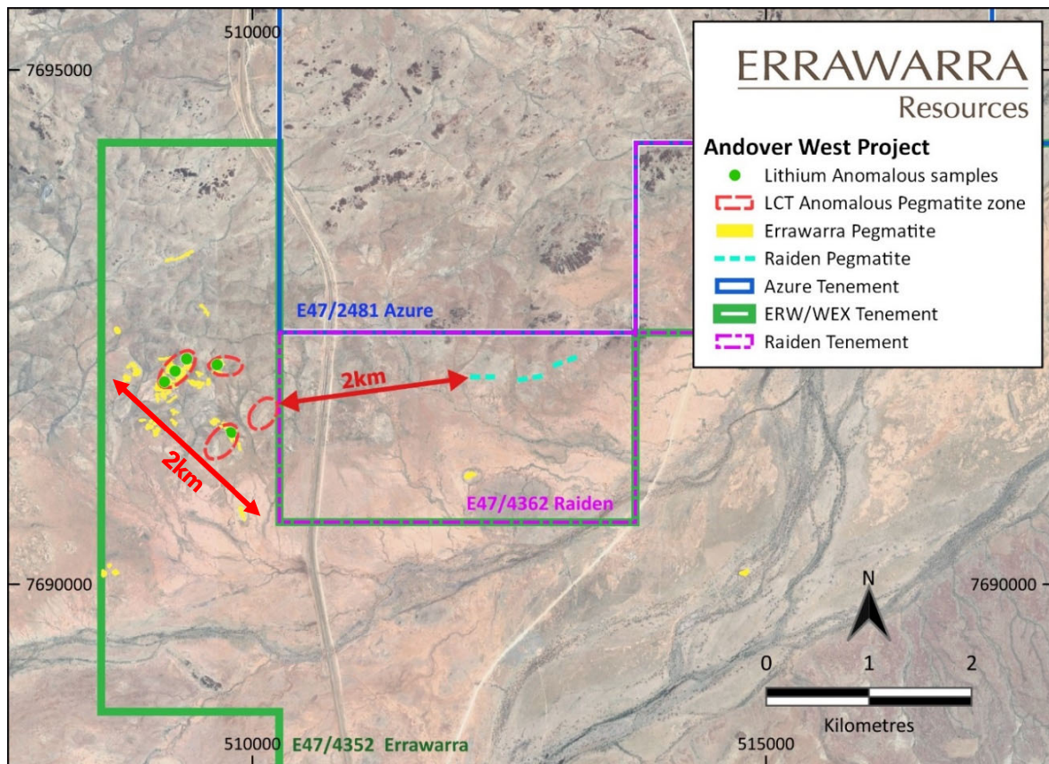
Figure 2. Location of rock chip collection points
