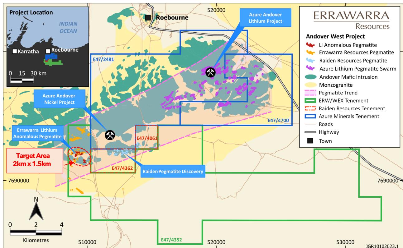
Figure 1. Andover West tenement and pegmatite target areas
