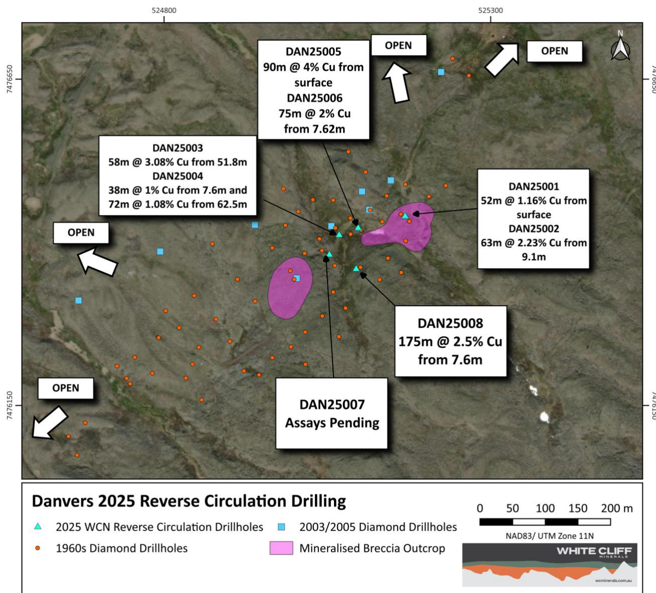
Figure 4 - Plan view of the Danvers licence area, showing drill hole collars of 1. (in cyan triangles) the RC drilling undertaken by the Company in 2025; 2. (in orange circles) the historic drilling that depicts the historic resource outline; and 3. (in blue squares) 2003 and 2005 drilling by Coronation that was designed to commence lateral step out and down dip drilling.
