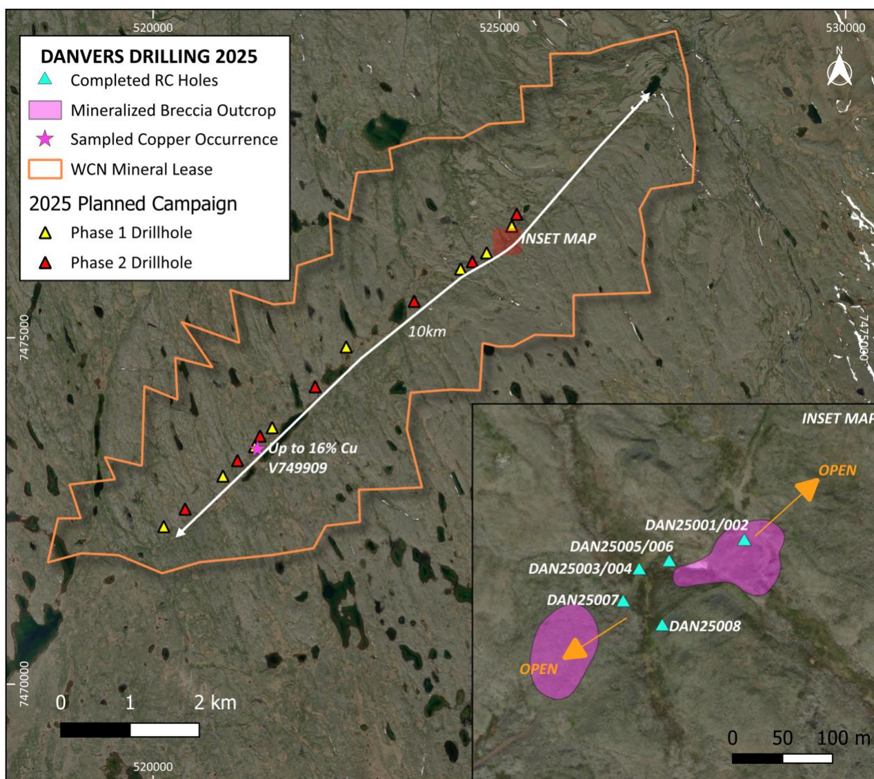
Figure 2 - Danvers Project. High grade historic copper occurrences present along a regional NE/SW trending fault zone for 10km. Inset map shows drillhole collars, covering only a fraction of the wider prospective corridor. The location of sample V749909 is marked by the pink star, where high grade copper is present on surface over 4.8km from drilling at Danvers.
