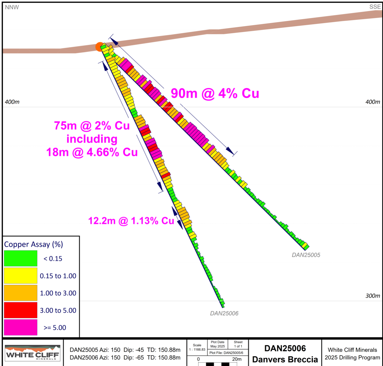
Figure 3 - Section of drillholes DAN25005 and DAN25006. Reported intercepts are drilled thicknesses, not true thicknesses.
