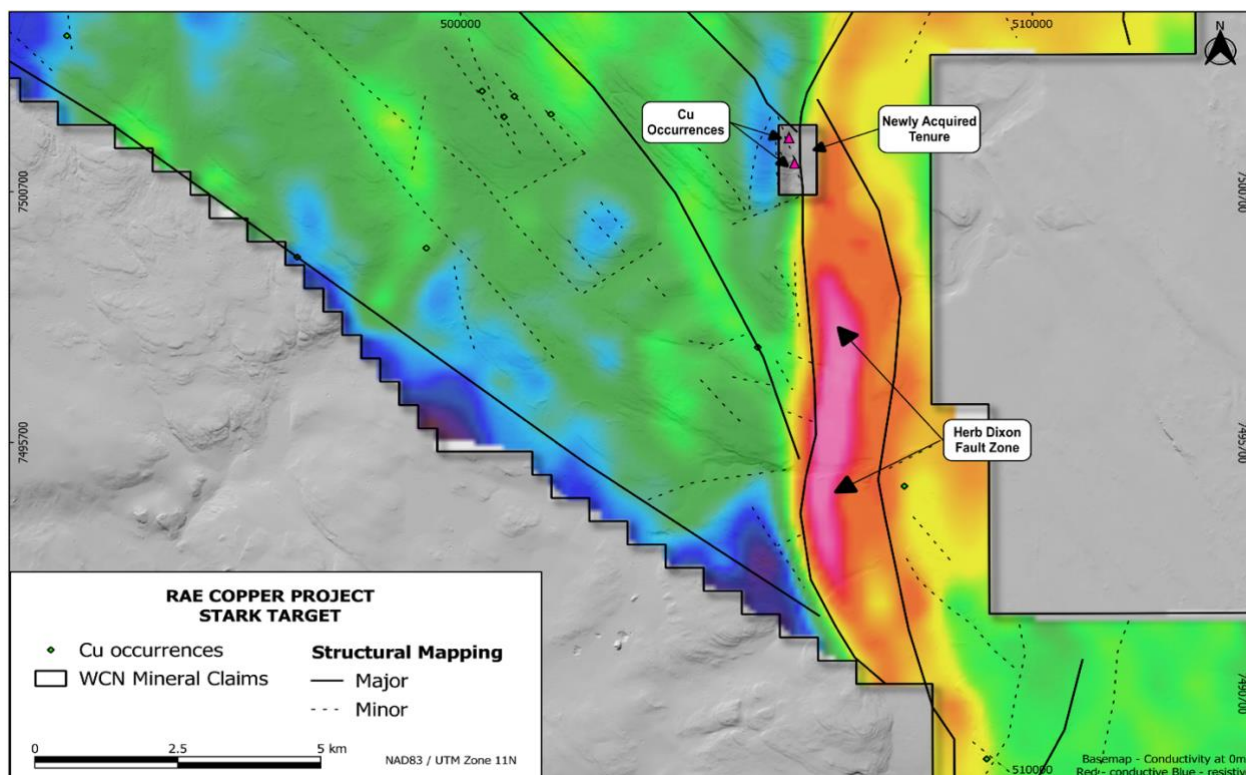
Figure 3 - Map of the southern Herb Dixon Fault Zone target named STARK showing high conductivity occupies a strong magnetic low within the fault zone that covers the Bornite Lake Copper Occurrence. Inverted resistivity response at 0m relative elevation.
