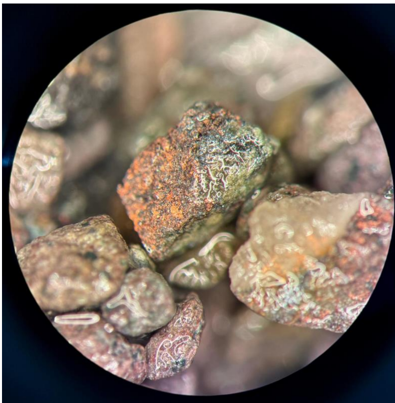
Figure 4 - Photograph of disseminated and vein-hosted chalcocite-native copper bearing RC chips from 99.06-100.58m depth in DAN26004. (Field of view approx. 10mm)
