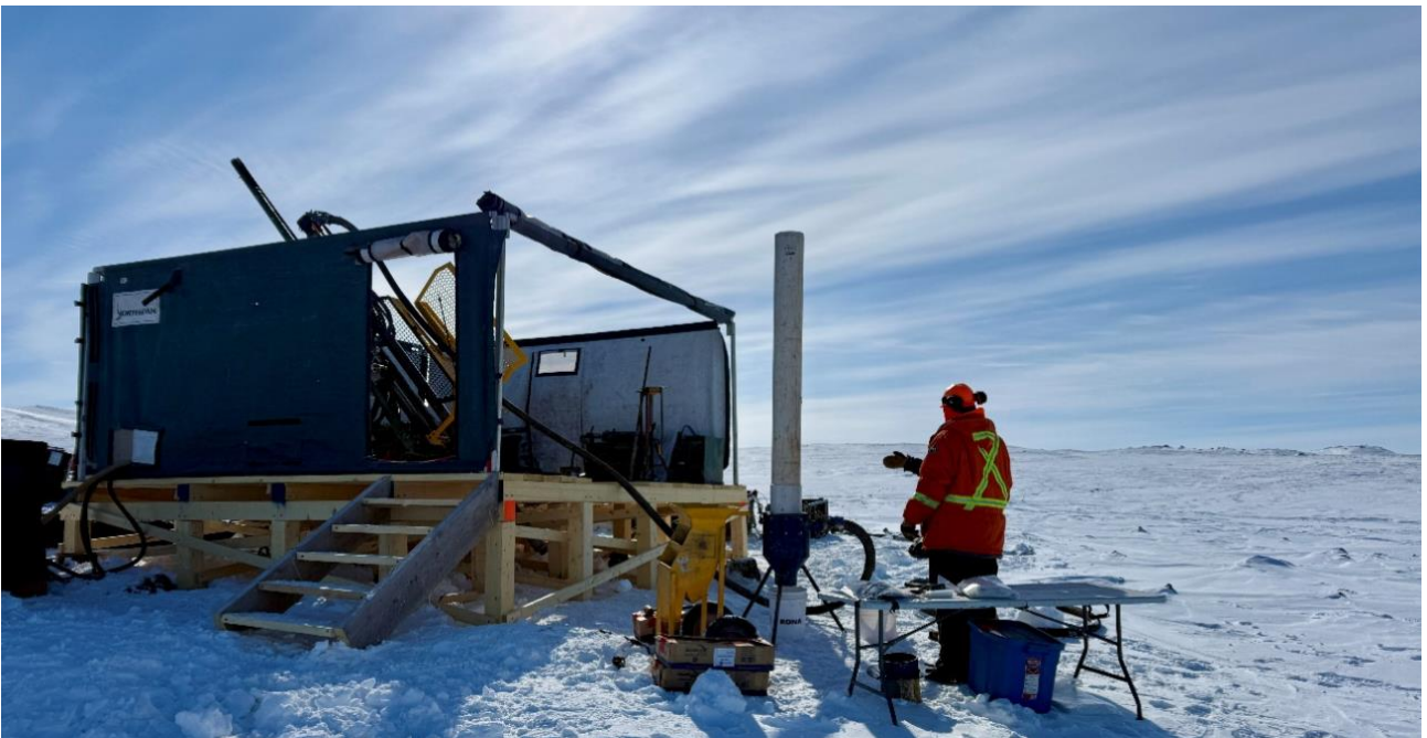
Figure 7 - Photograph of reverse circulation drilling rig on DAN26002 targeting the Teshierpi Fault Zone
