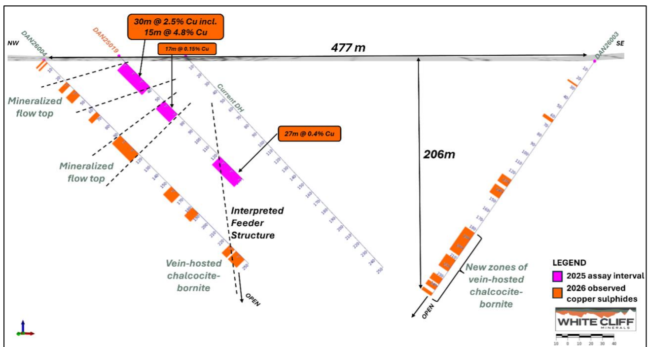
Figure 1 - Section through drillholes DAN25019, DAN26003 and DAN26004. New zones of observed copper sulphides depicted with orange rectangles downhole, which correlate to the assay intervals from the 2025 drillhole DAN25019. Current DH is DAN26006 and is currently being drilled. Both flow top replacement mineralisation and vein hosted chalcocite-bornite is reported from drillholes, refining the model and confirming the Teshierpi Fault Zone as a broad zone of copper mineralisation.
