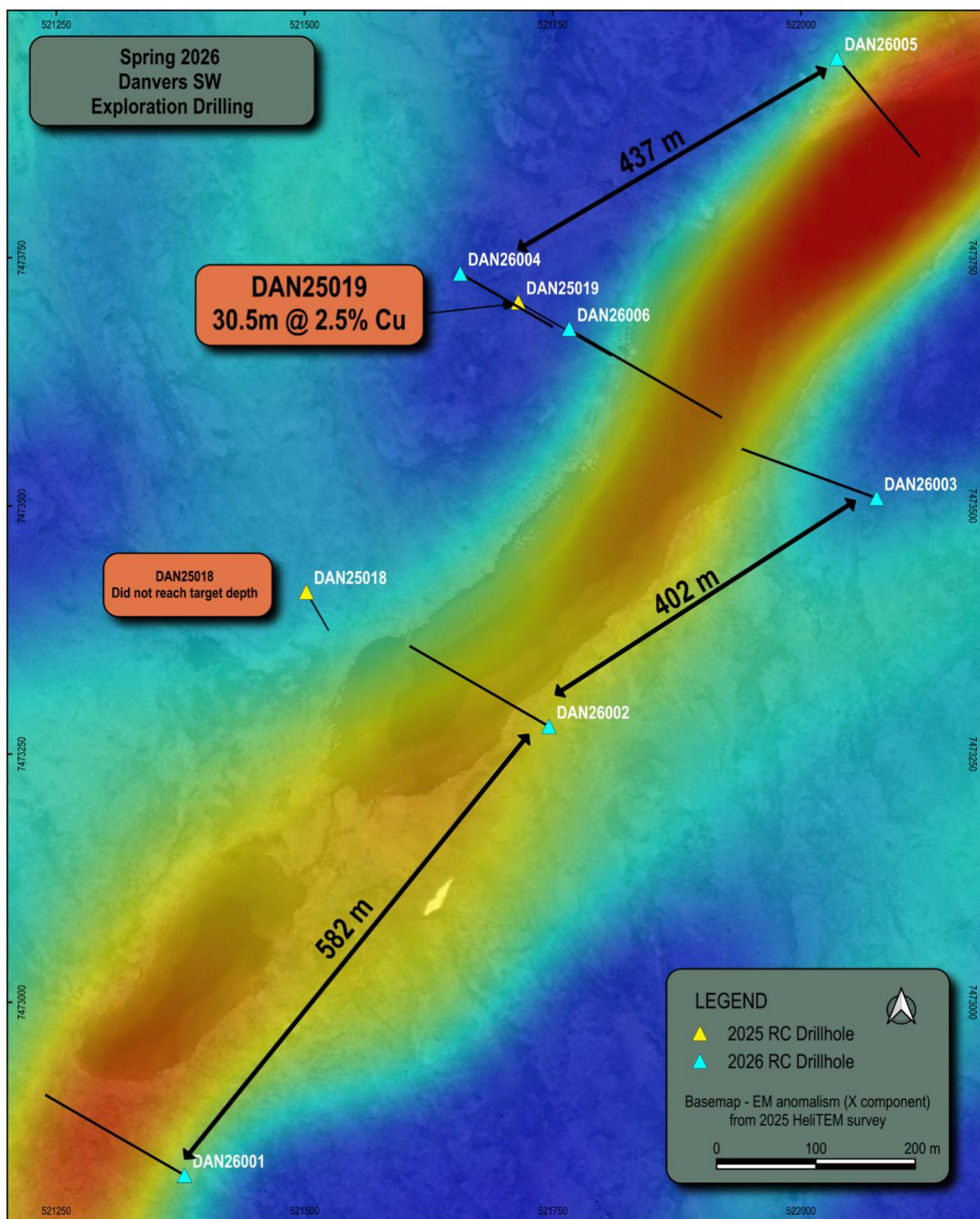
Figure 8 - Map of early time EM channels X component, RGB of 3 channels converted to single band pseudo-colour. Red areas represent peak conductivity, blue areas are more resistive. Drillholes from 2025 discovery of Danvers II (DAN25019) and 2026 holes are depicted. NAD83 UTM Zone 11N.
