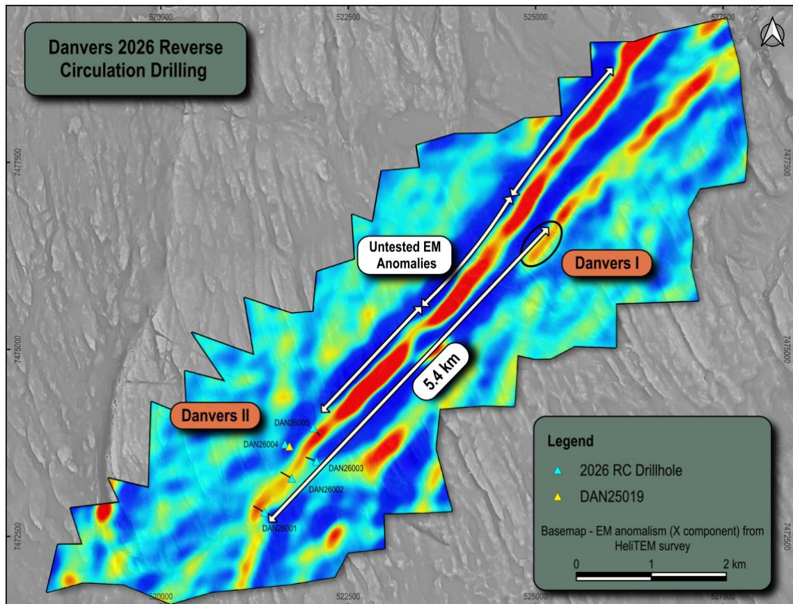
Figure 2 - Danvers 2026 drilling campaign to date -overlaid against map of early time EM channels X component, RGB of 3 channels converted to single band pseudo-colour. Red areas represent peak conductivity, blue areas are more resistive.
