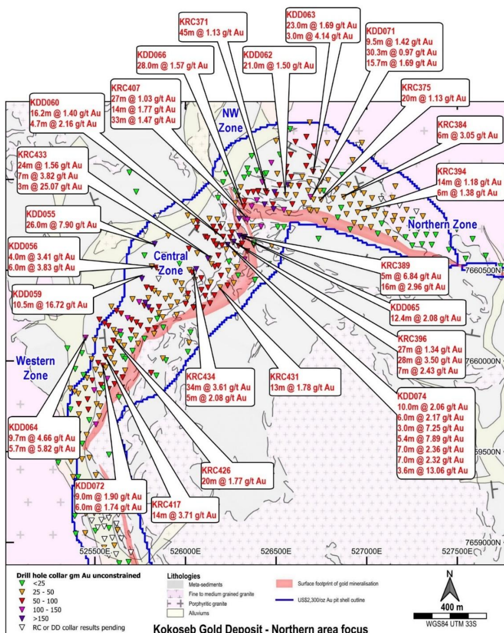
Figure 6 – Drill hole locations, focused at the northern area of Kokoseb, location of the long section and cross sections of this announcement and most significant intercepts on drill holes reported during the July quarter 7
