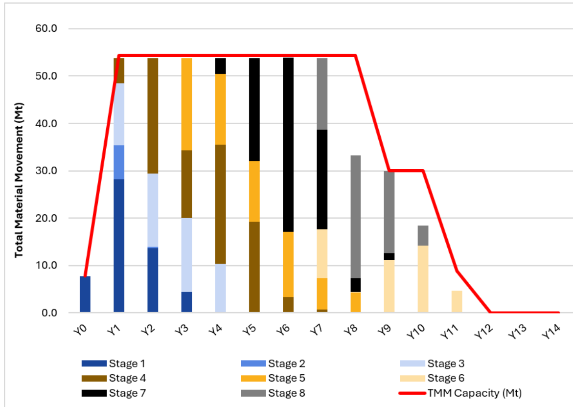
Figure 8.22: Annual Mining Movement by Pit Stage
