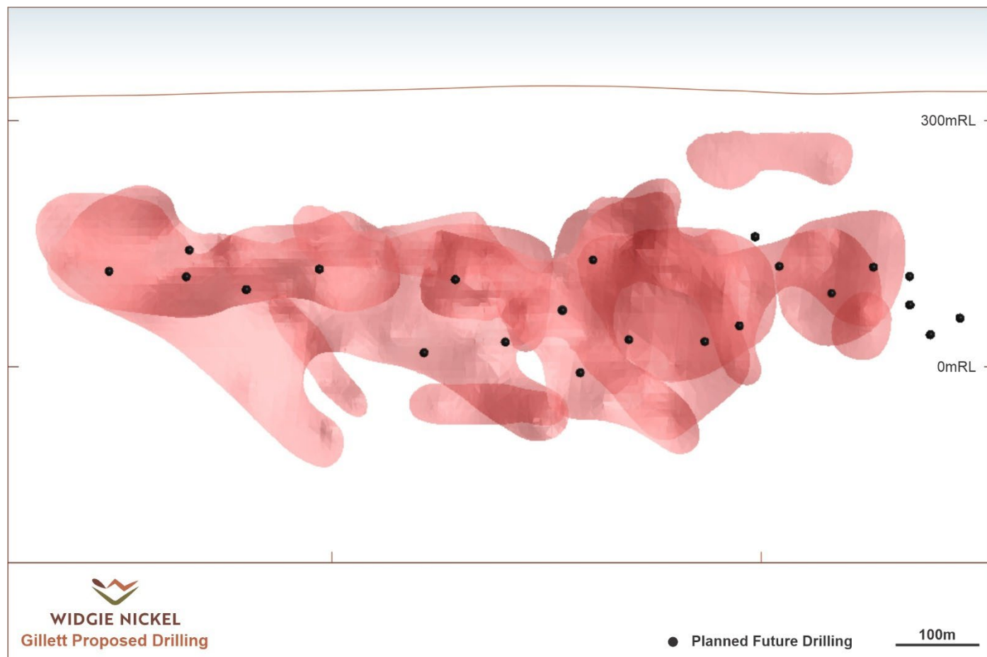
Figure 9 - Long section of the Gillett Mineral Resource and targeted future drilling.
