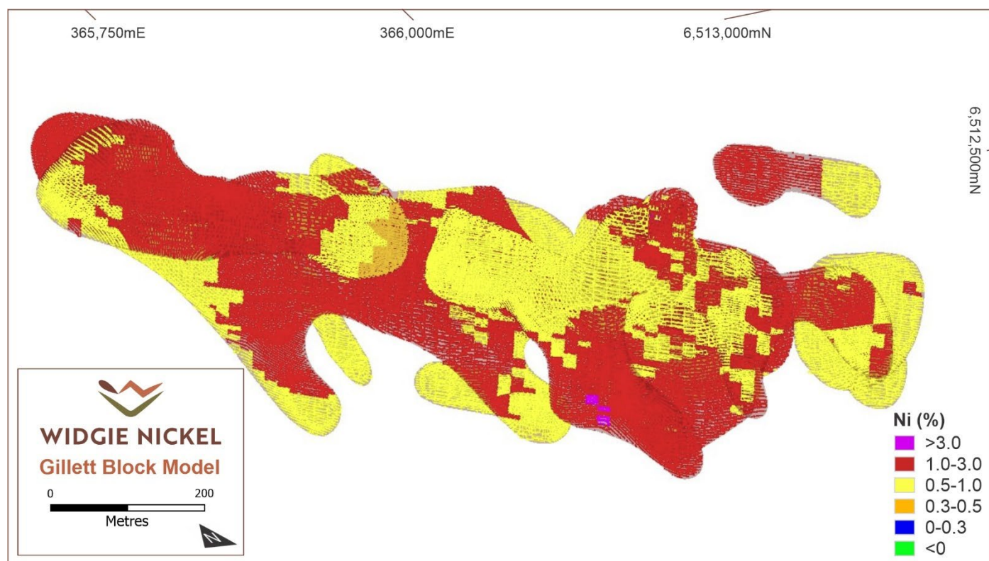
Figure 7 - 3D view of the 2023 Gillett Mineral Resource block model coloured by nickel grade
