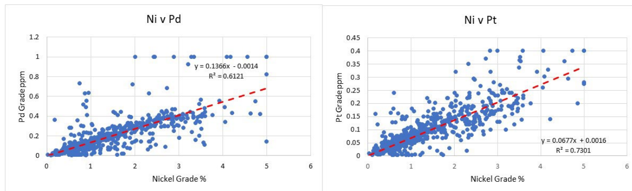
Figure 6 - Plots of composites used in the estimate illustrating the correlation between Nickel and Palladium and Platinum
