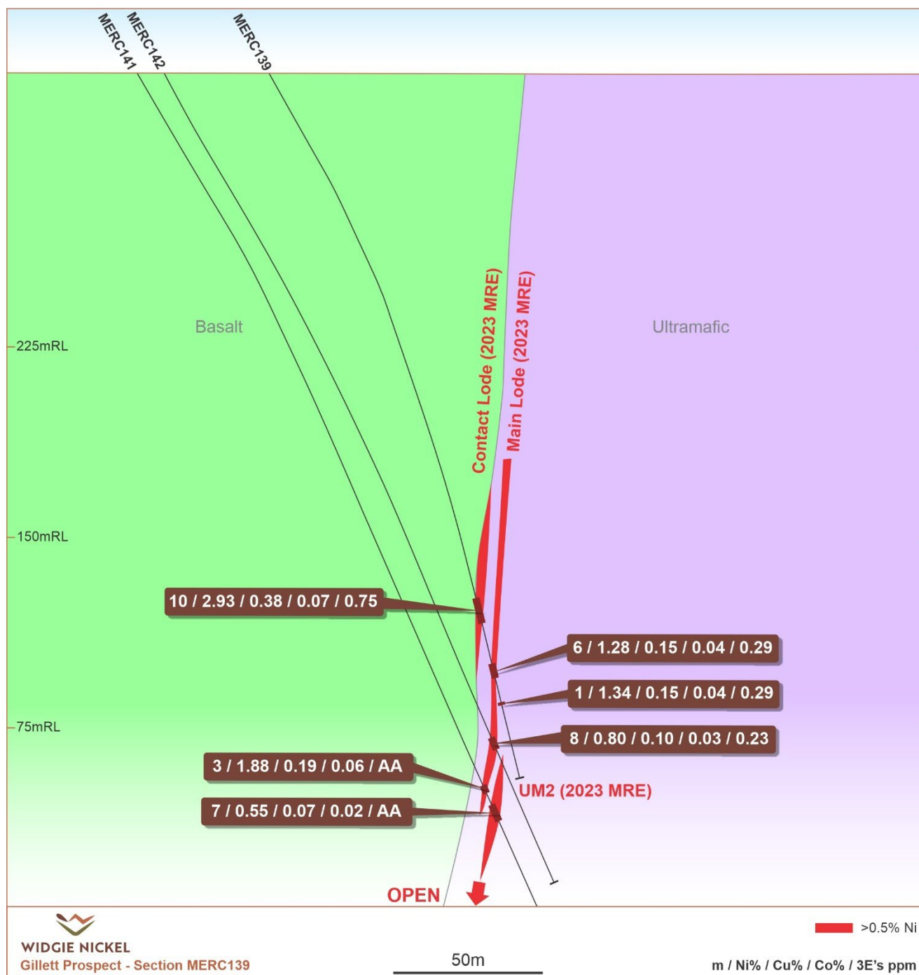
Figure 3 - Cross Section with recent drill intercepts of the Gillett Nickel mineral resource. The mineralisation is in the ultramafic of an overturned limb of an anticline under a hanging wall of basalt. All three mineralised horizons are shown
