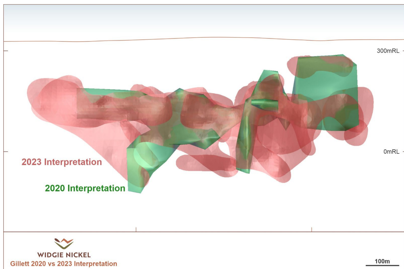
Figure 8 - Long section with current 2023 mineralised envelope (red) compared to the 2020 interpretation (green)
