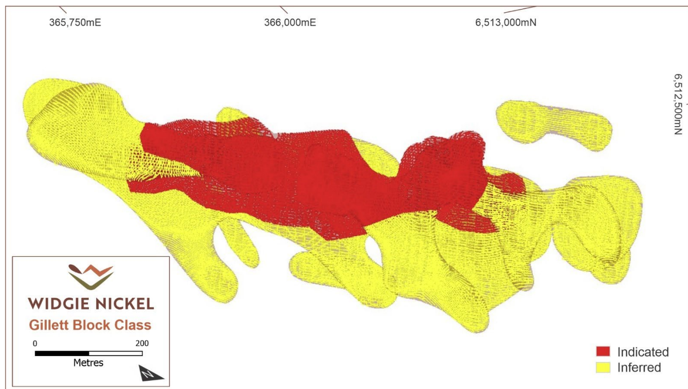
Figure 5 – View looking north-east showing model classification
