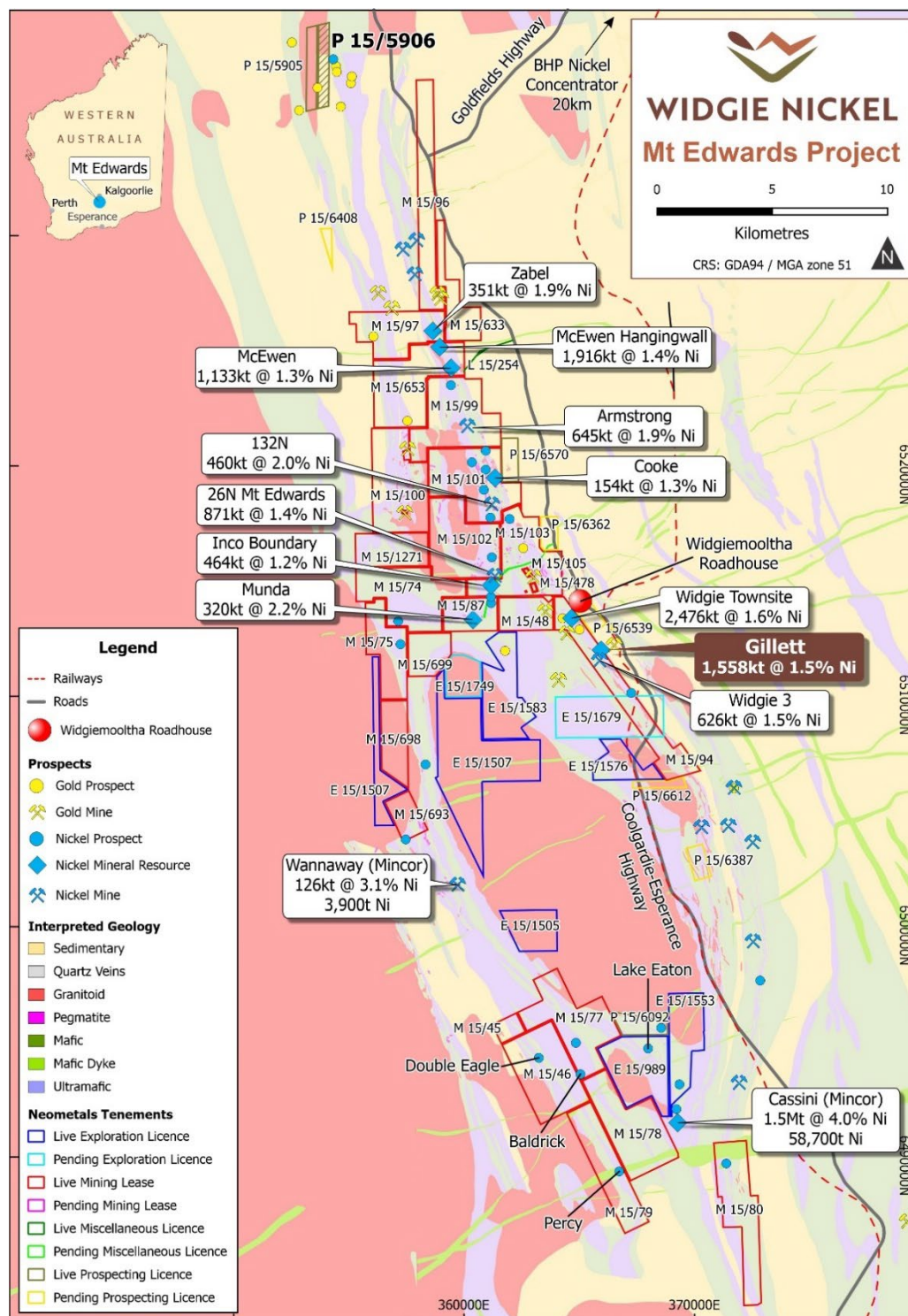
Figure 1 - Mt Edwards Project tenure over geology, with the Gillett Mining Lease M15/94 located within the Mt Edwards Project. Other Mineral Resources and prospects are displayed. Widgie Nickel hold 100% nickel rights for all live tenements shown above.
