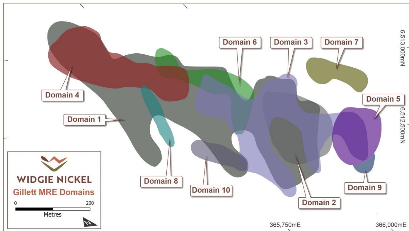
Figure 4 - View looking NE showing Gillett Mineral Resource domains
