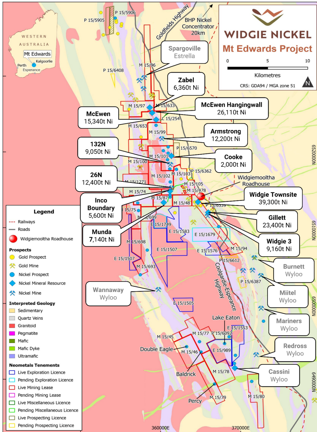
Figure 2 Mt Edwards nickel deposits (1% Ni Resource cut-off)
