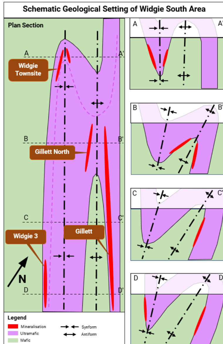
Figure 4 Schematic of Widgie South geology and mineralisation positions
