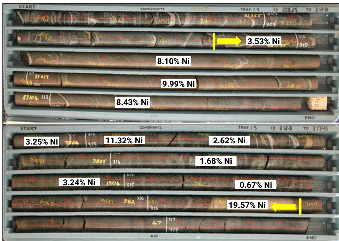
Figure 1 23MERC073 Individual assay results from massive to matrix sulphide mineralisation
