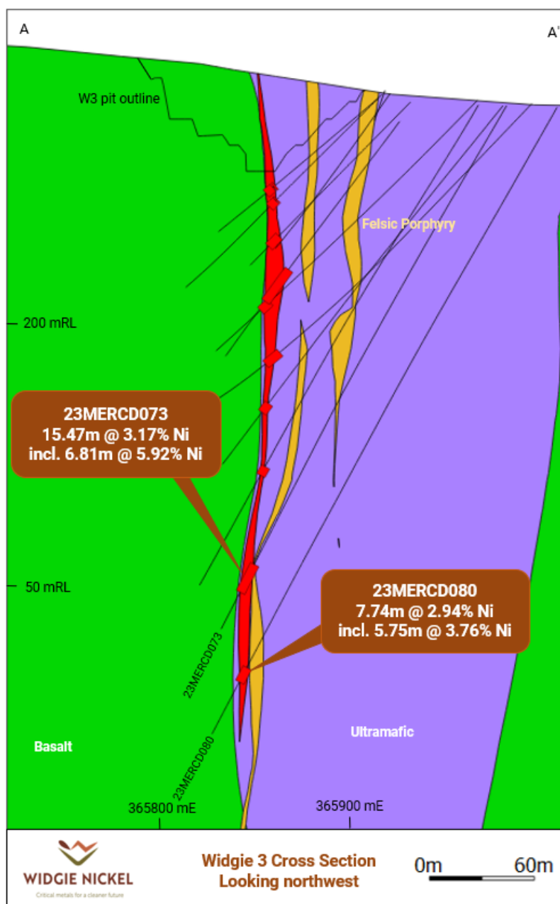
Figure 6 23MERCD073 and 23MERCD080 drill section
