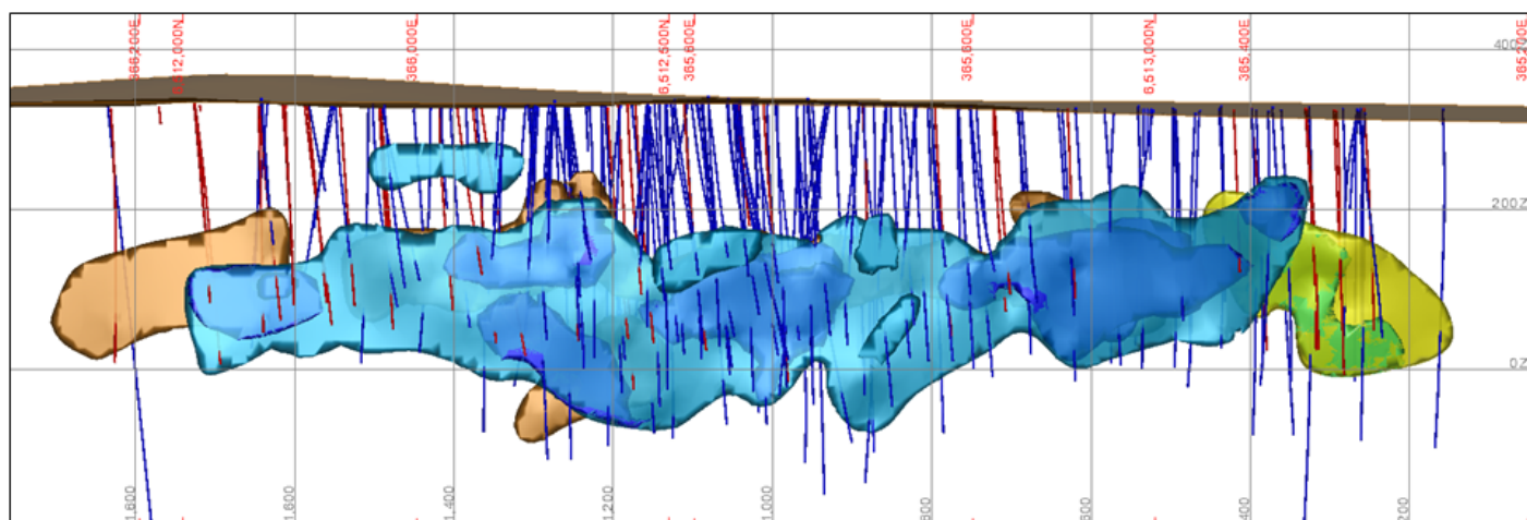
Figure 7: Gillett Mineralisation Interpretation and Drilling (red trace 2022-2023 drilling) – looking South-West
