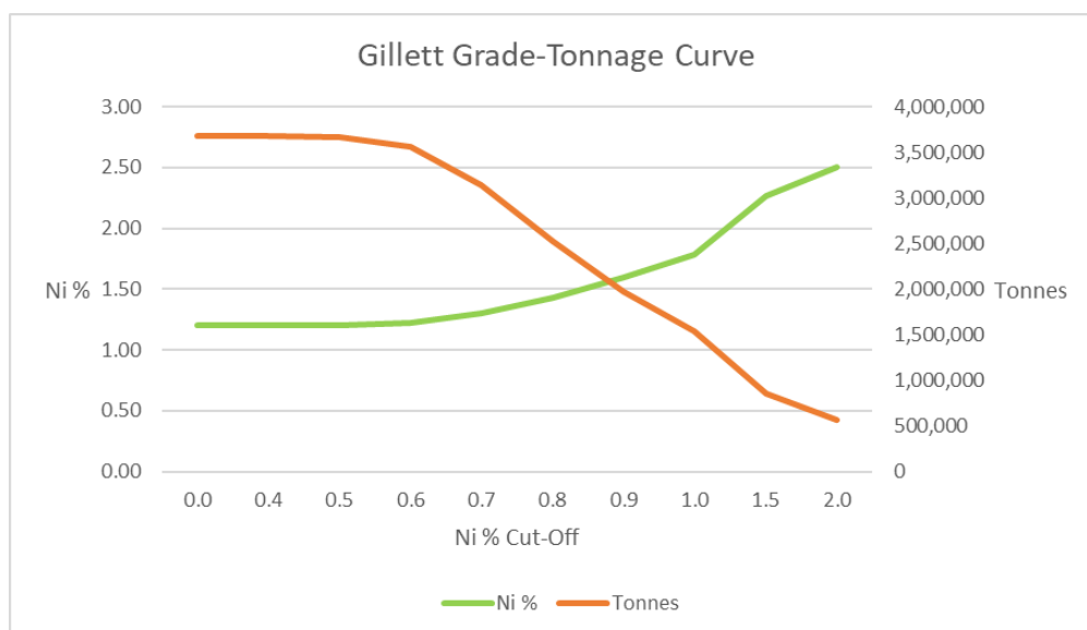
Figure 1: Gillett grade-tonnage curve
