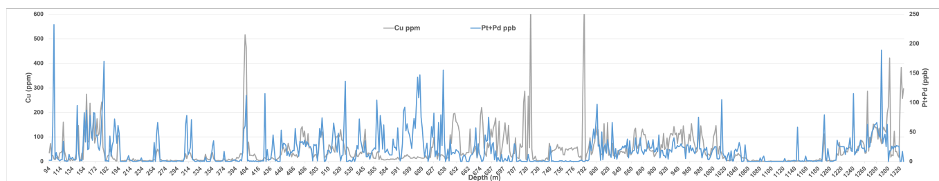
Figure 3: MTD023 Cu and Pt+Pd
