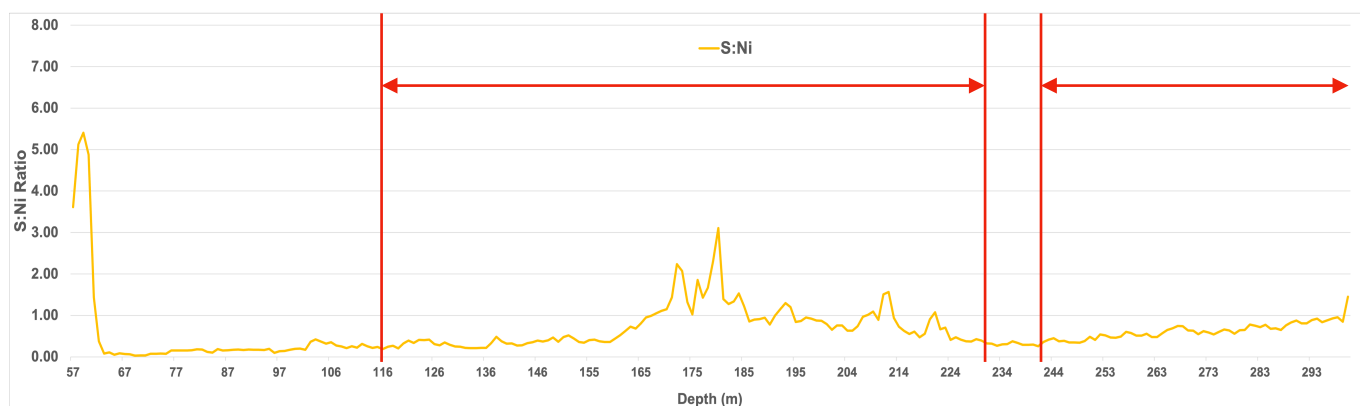
Figure 5: MTRC048 S:Ni Ratio
