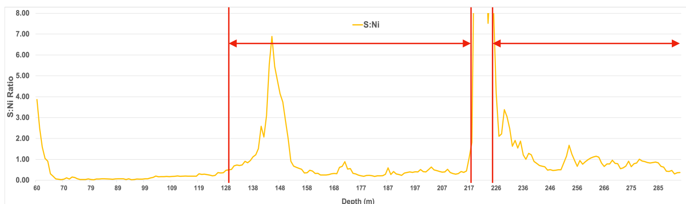
Figure 9: MTRC050 S:Ni Ratio
