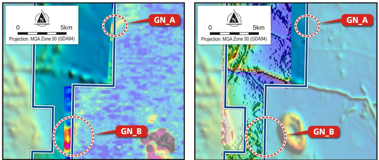
Figure 2: LHS shows SkyTEM (high moment Ch35) with anomalies GN_A and GN_B. RHS shows 80m magnetic TMI 1VD image with north shade at same scale. Refer to Figure 1 for map legend.
