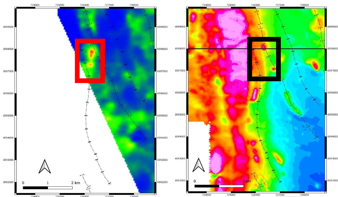
Figure 5: SkyTEM Z20 Band and TMI Magnetics over target GN_E
