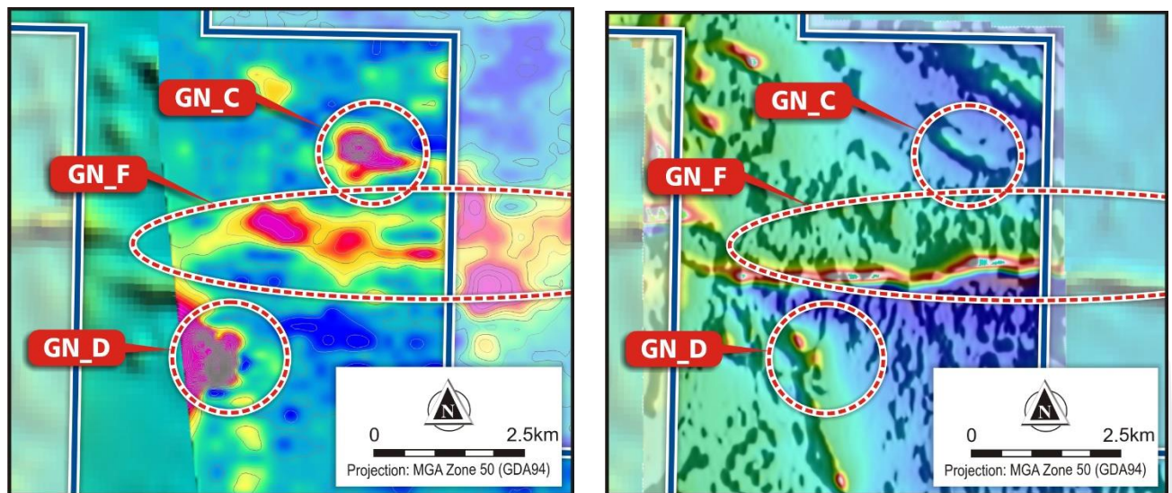
Figure 3: LHS shows SkyTEM (high moment Ch35) with anomalies GN_C, GN_D and GN_F. RHS shows 80m magnetic TMI 1VD image with north shade at same scale. Refer to Figure 1 for map legend.
