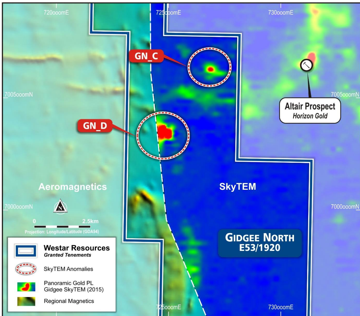
Figure 6: Location of Westar SkyTEM anomalies in relation to Horizon Gold's Altair Prospect
