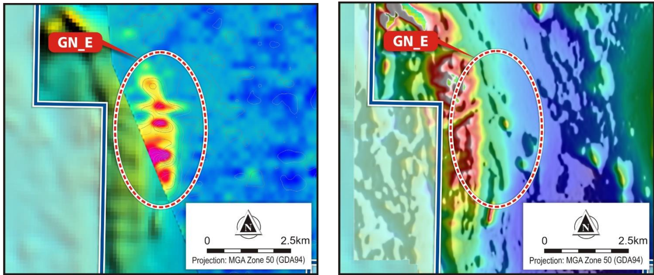
Figure 4: LHS shows SkyTEM (high moment Ch35) with anomaly GN_E. RHS shows 80m magnetic TMI 1VD image with north shade at same scale. Refer to Figure 1 for map legend.
