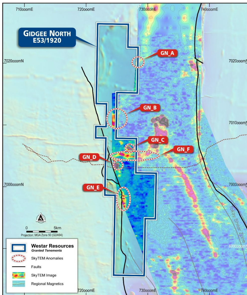
Figure 1: SkyTEM (high moment Ch35) shown with tenement boundary and anomalies identified.
