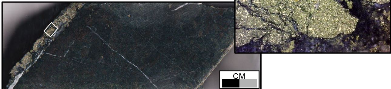
Figure 4: SPD048 – 551.5 m, 37.85 g/t Au. Pyrite-quartz-carbonate-chlorite-magnetite-Au vein reactivated with later carbonate veining in basaltic andesite.
