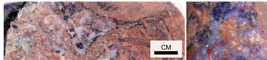
High grade gold from Consols Zone 701 m. 120g/t Au. Quartz-magnetite-gold-pyrite breccia associated with strong potassic alteration (SPD027)
