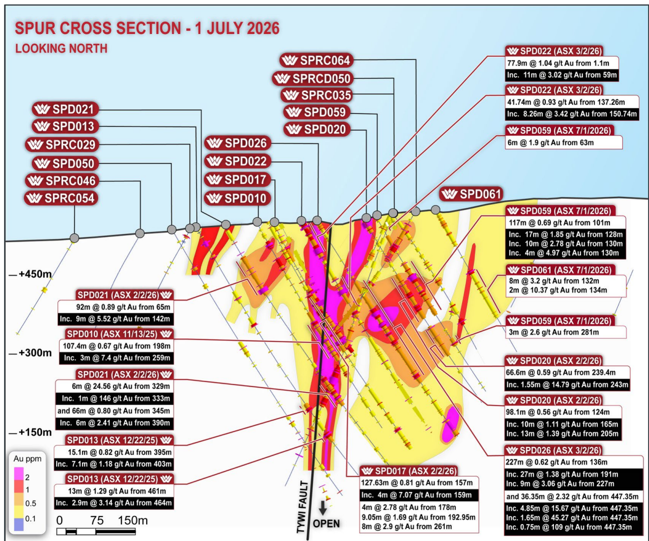
Figure 4: Spur Gold Zone Cross Section
