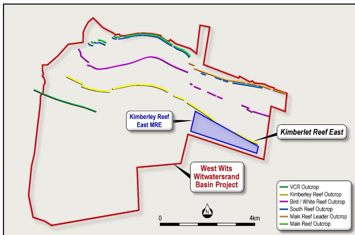
Figure 1: Outcrop of the significant Gold producing Conglomerates within the WBP
