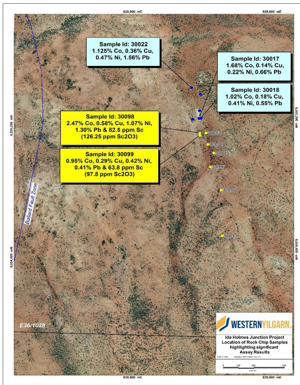
Figure 1 – Location Map over E36/1028 highlighting the high-grade Co-Cu-Ni-Pb-Sc rock chip results
