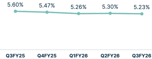
Portfolio NIM
