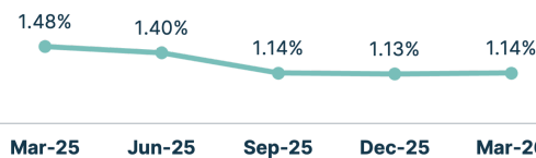
90+ day arrears
