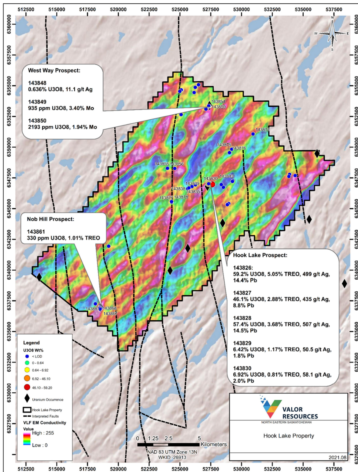
Figure 3: Significant and anomalous sample results across the Hook Lake Property
