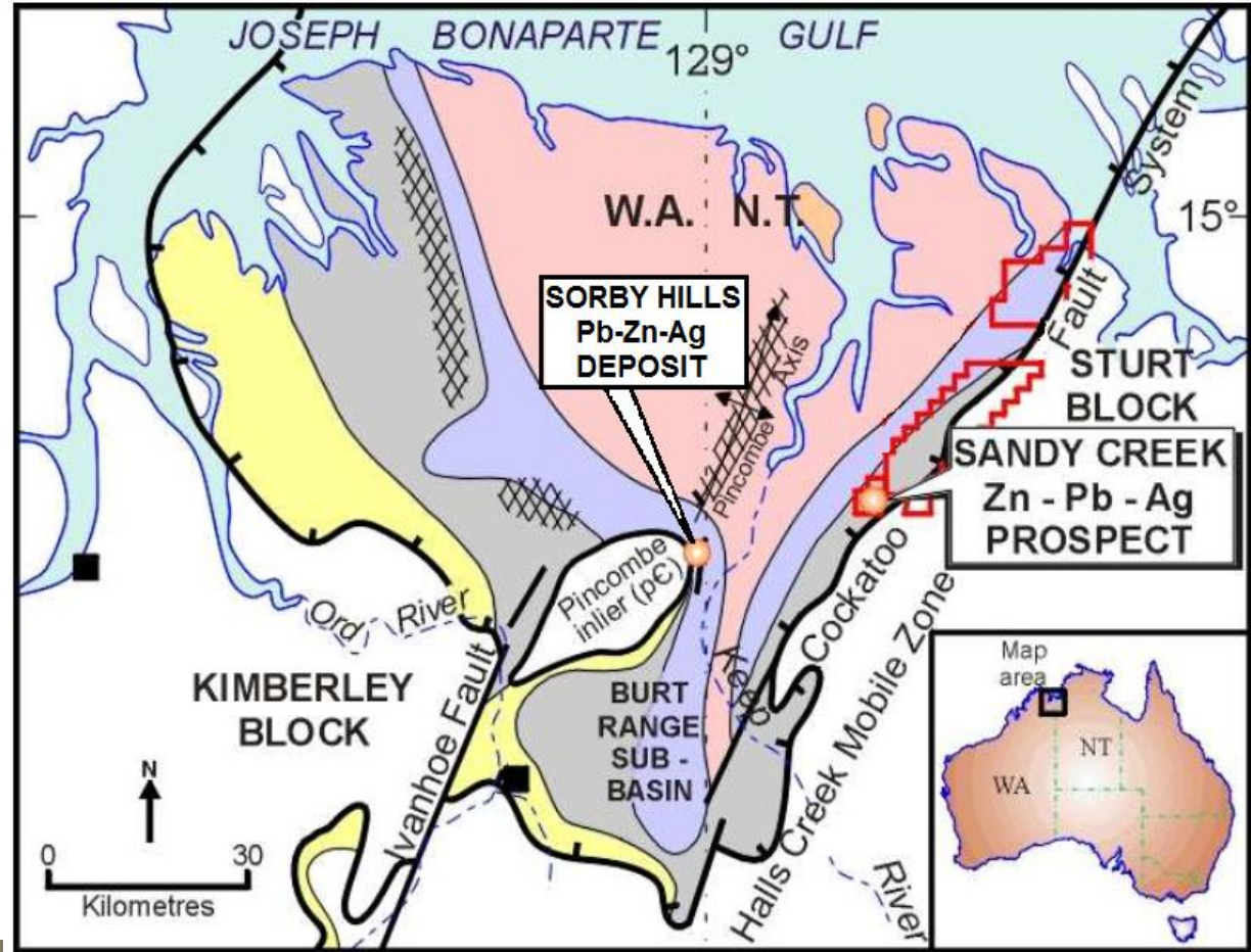
Geological setting of the Sandy Creek and Sorby Hills Mineral Resources
