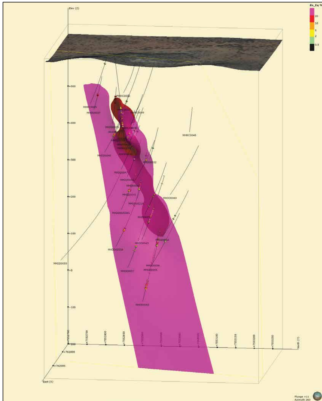
Figure 2. Hendrix Resource wireframes and drilling looking west.
