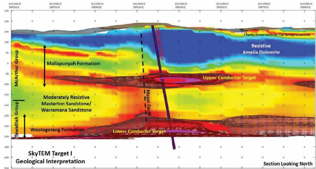
Figure 10. Conductor targets in the Mallapunyah and Wollgorang Formations for Hole MCDD0005.
