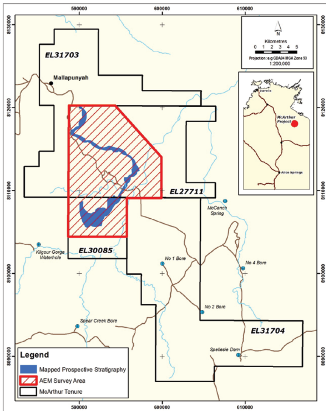
Figure 8. Location of the McArthur River tenure in relation to the mapped prospective stratigraphy and showing the location of the detailed SkyTEM survey completed in August 2017.
