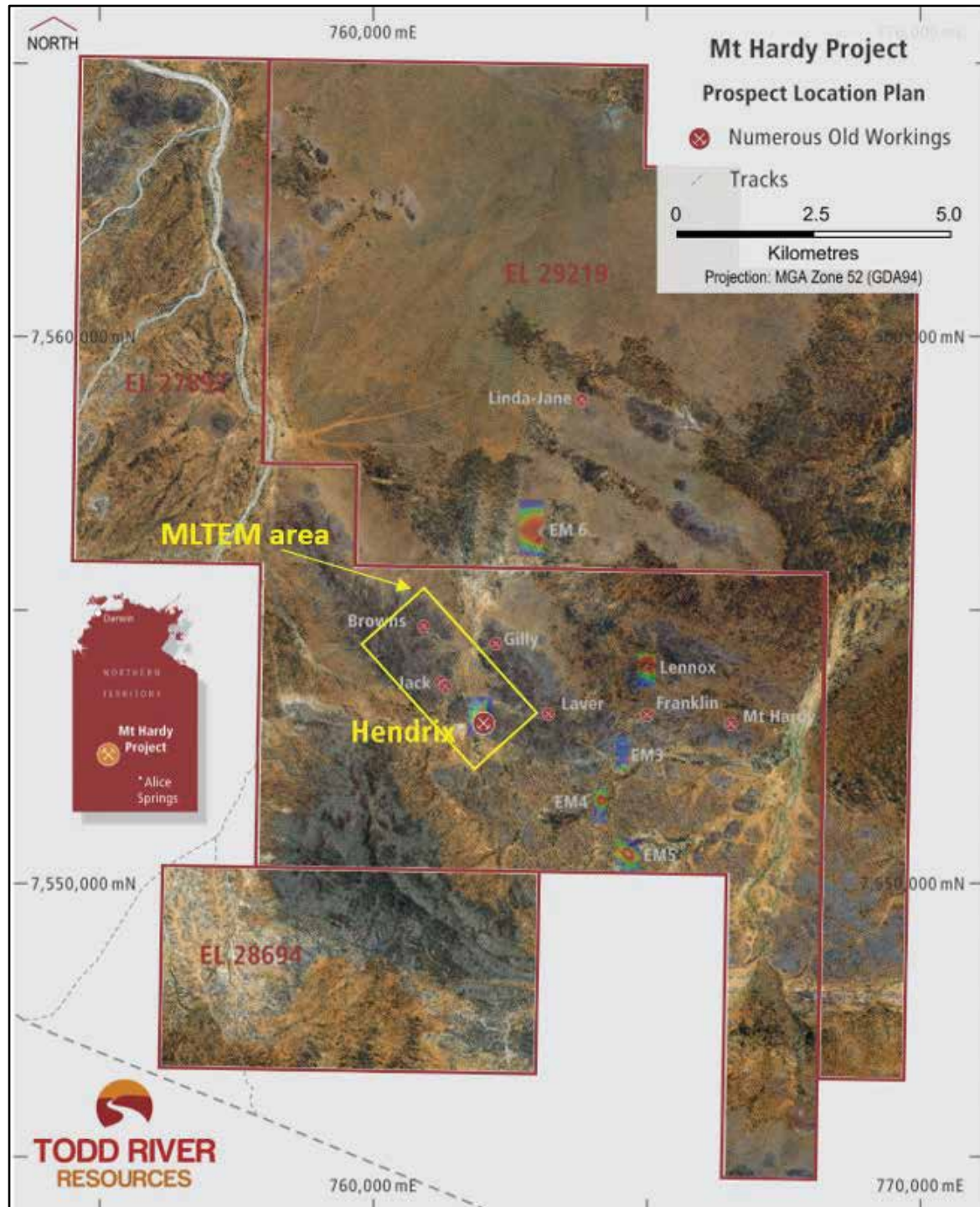
Figure 6. Location of MLTEM survey area around Hendrix and north to Browns.
