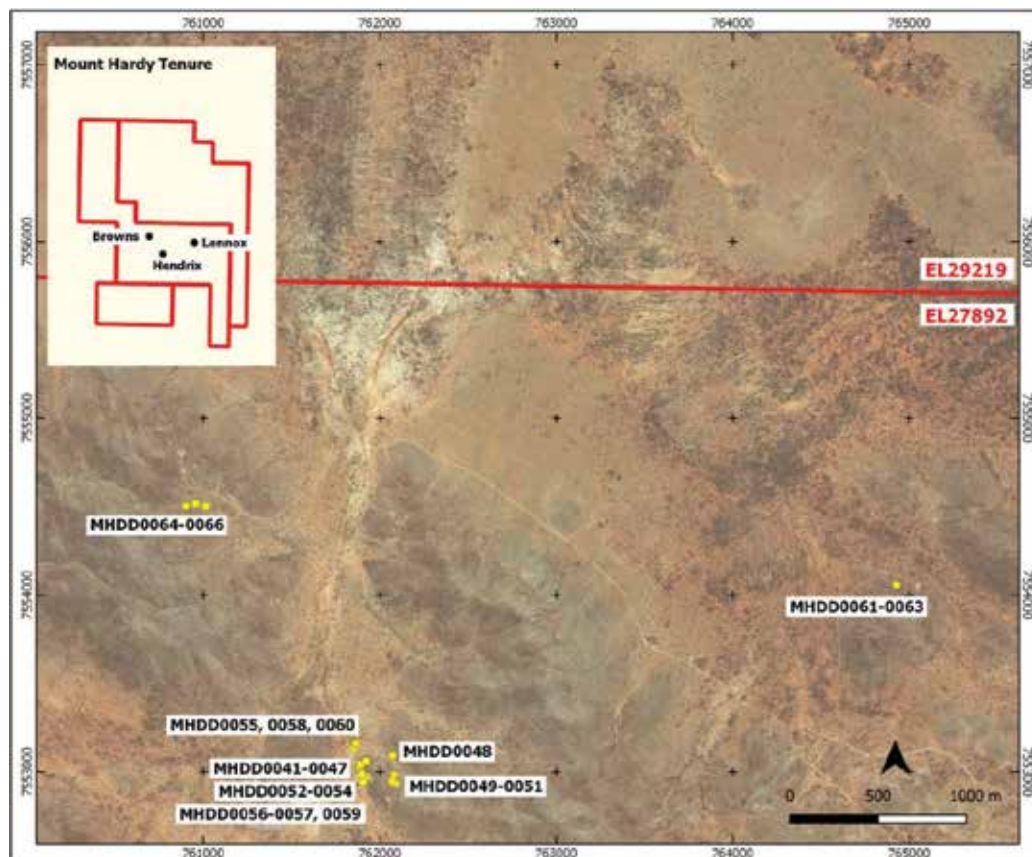
Figure 4. 2018 Mt Hardy Project drill collar plan.
