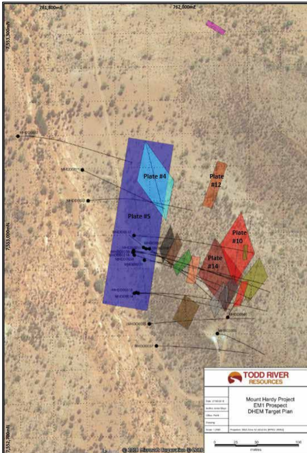
Figure 5. Conductive plates identified during downhole TEM surveying of holes at Hendrix.
