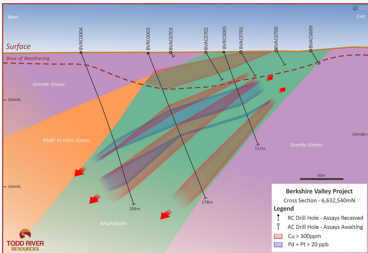
Figure 6 – Cross section showing the thickness of the amphibolite unit and distribution of the copper and PGE anomalous zones.
