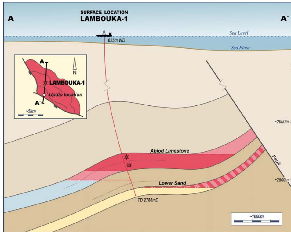
Figure 5: Schematic Lambouka Cross Section with Top Abiod Structure Map
