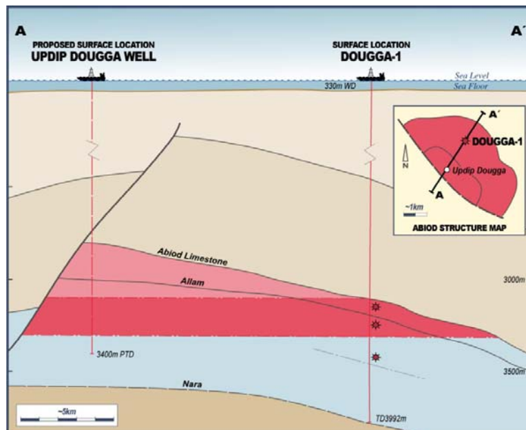
Figure 4: Schematic Dougga Cross Section with Top Abiod Structure Map
