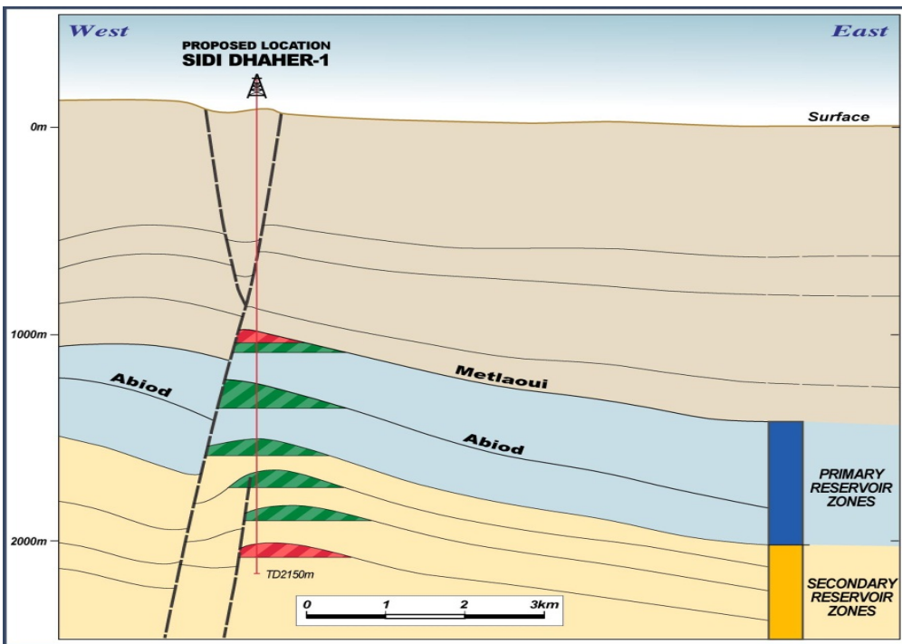
Figure 2: Schematic Sidi Dhaher Cross Section showing 6 potential reservoir zones
