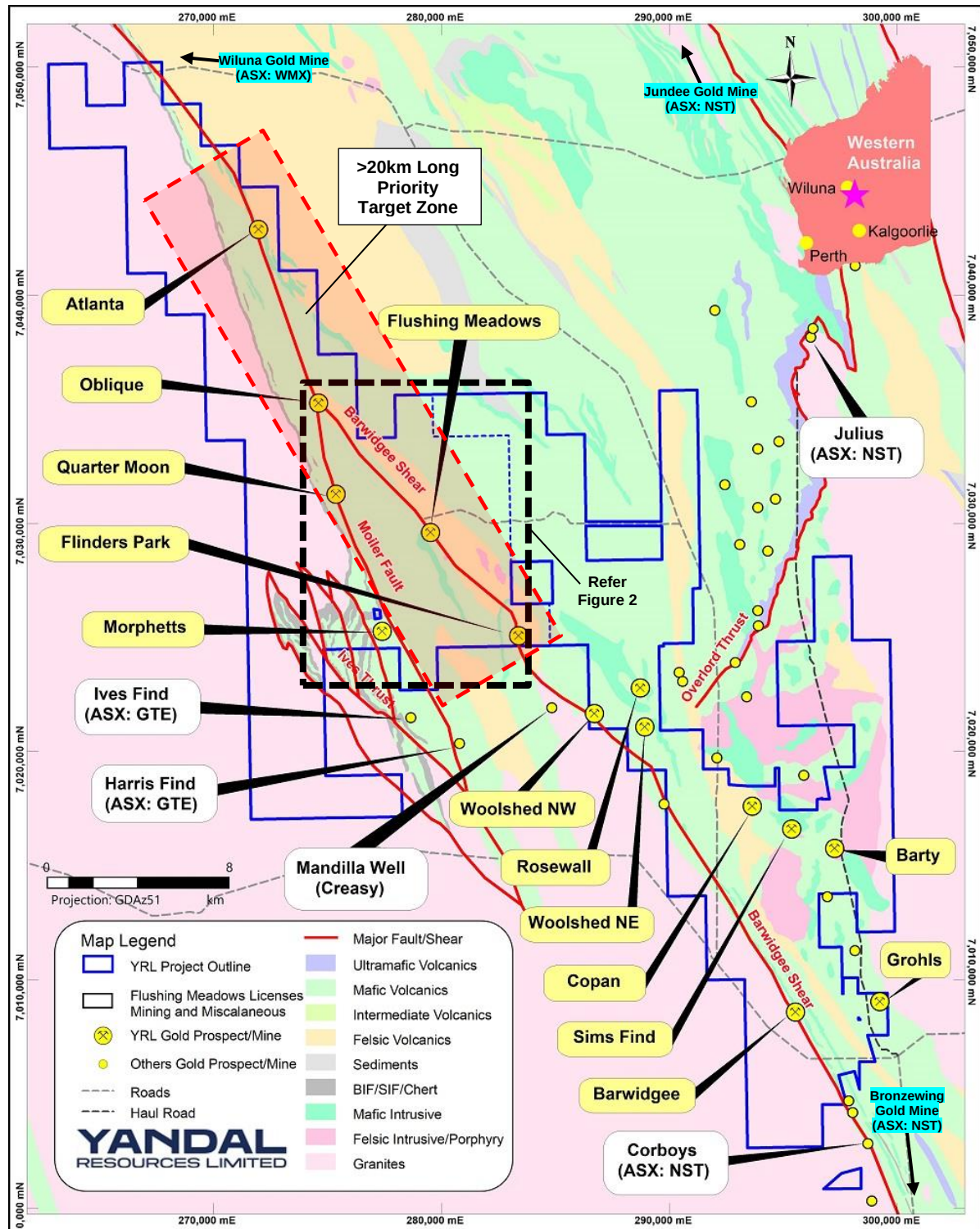
Figure 1 – Location map of key prospects within the Company’s Ironstone Well and Barwidgee gold projects in relation to nearby third party gold mines, project tenure and regional geology. Note the >20km long Flinders Park to Atlanta priority target zone highlighted with red dashed lines (Refer to Figure 2 for detailed map).
