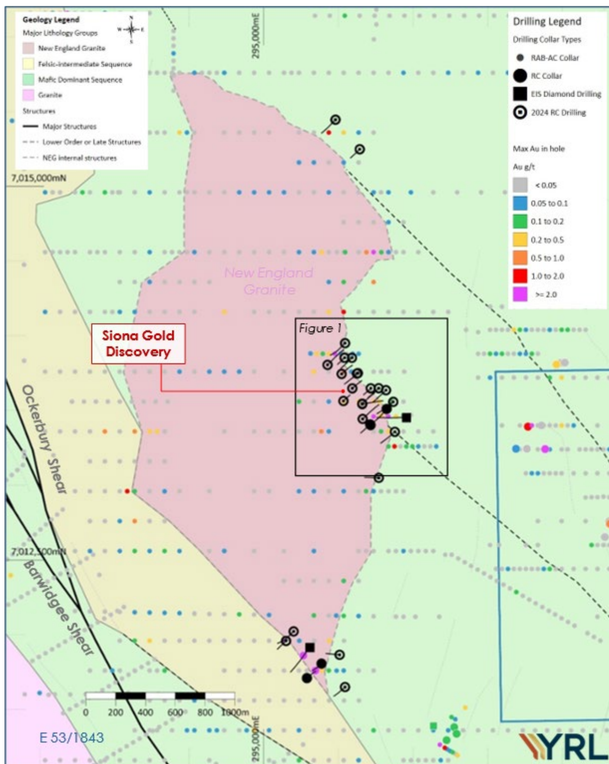
Figure 3: A Collar plan for the broader New England Granite area displaying all drilling collars, colour-coded by max Au in hole (g/t Au), overlying a simplified interpretation of bedrock geology. Note interpreted northwest trending structures internal to the New England Granite.
