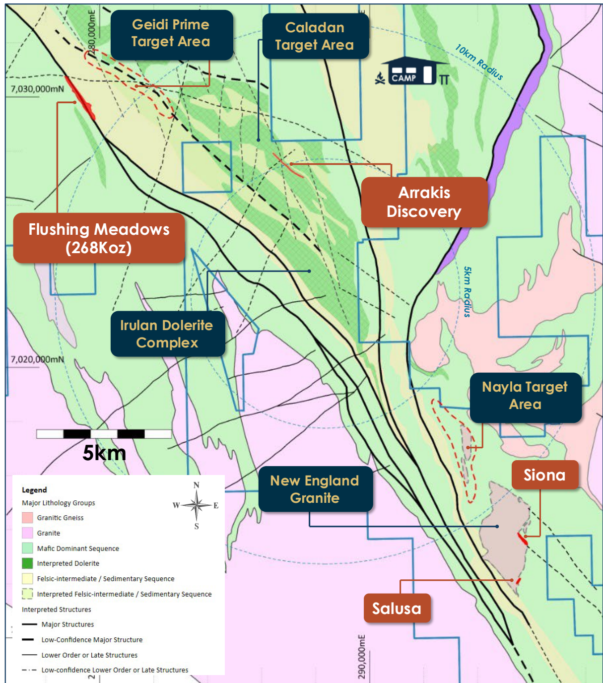
Figure 11: Yandal Resource exploration target areas and prospect locations within the northern Yandal Greenstone Belt. The Arrakis Prospect is located within the Caladan target area.
