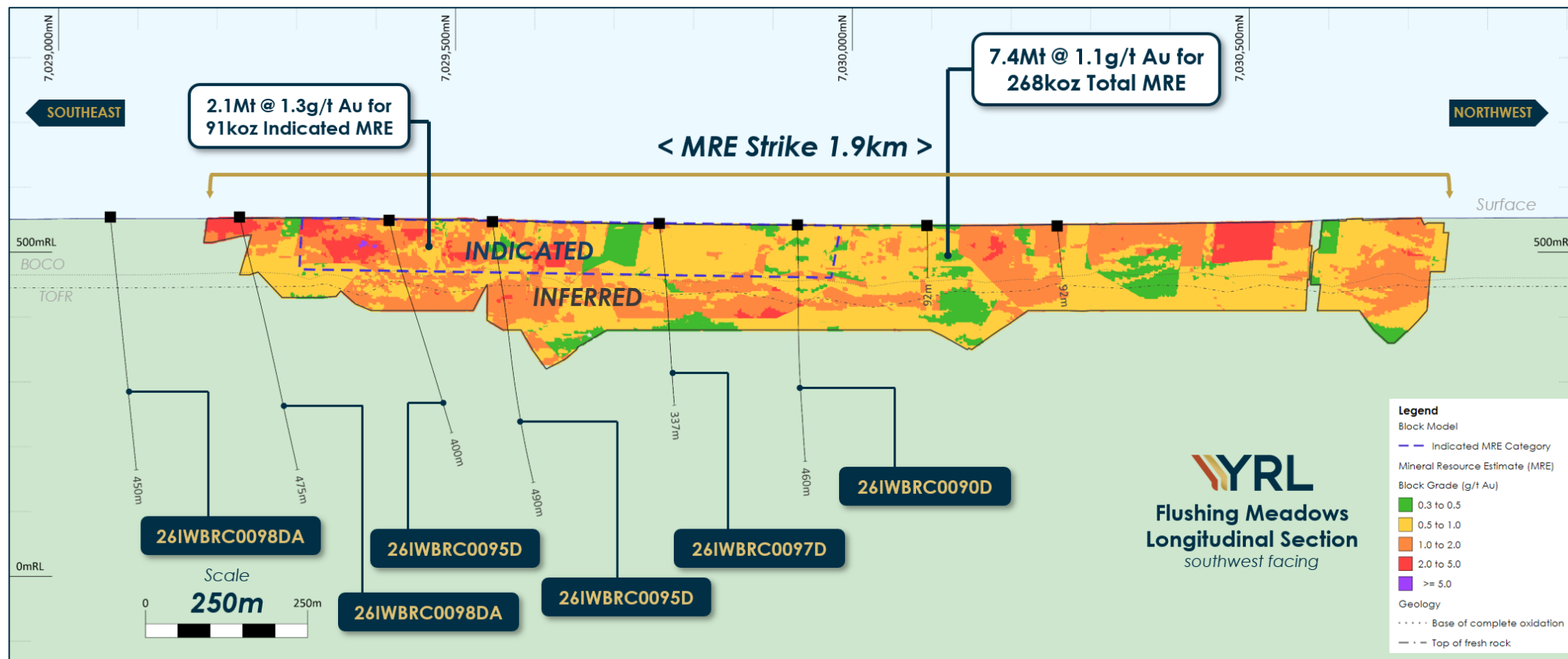
Figure 8: A southwest facing longitudinal section displaying the Flushing Meadows MRE outline (see ASX release 4 November 2020) and the drill strings of completed diamond drilling below the MRE.
