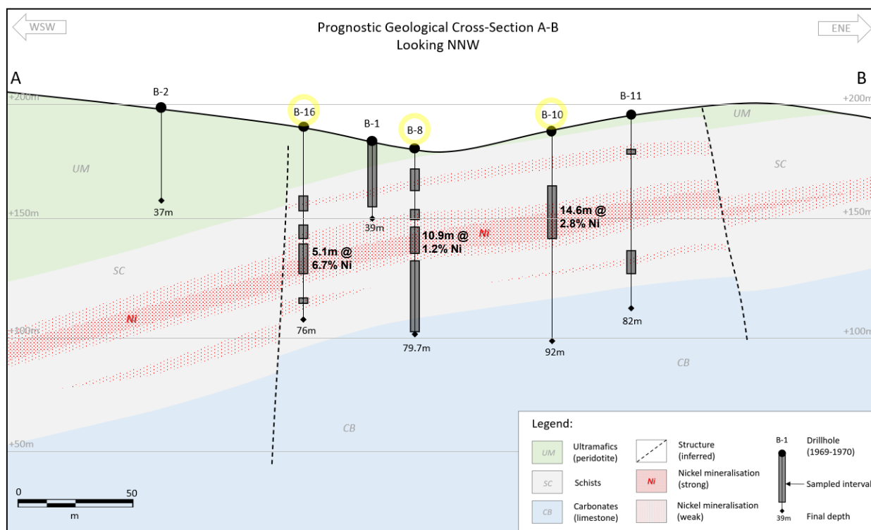
Figure 3: Sockovac (Petrovo) cross-section showing historical drill holes with interpreted geology
