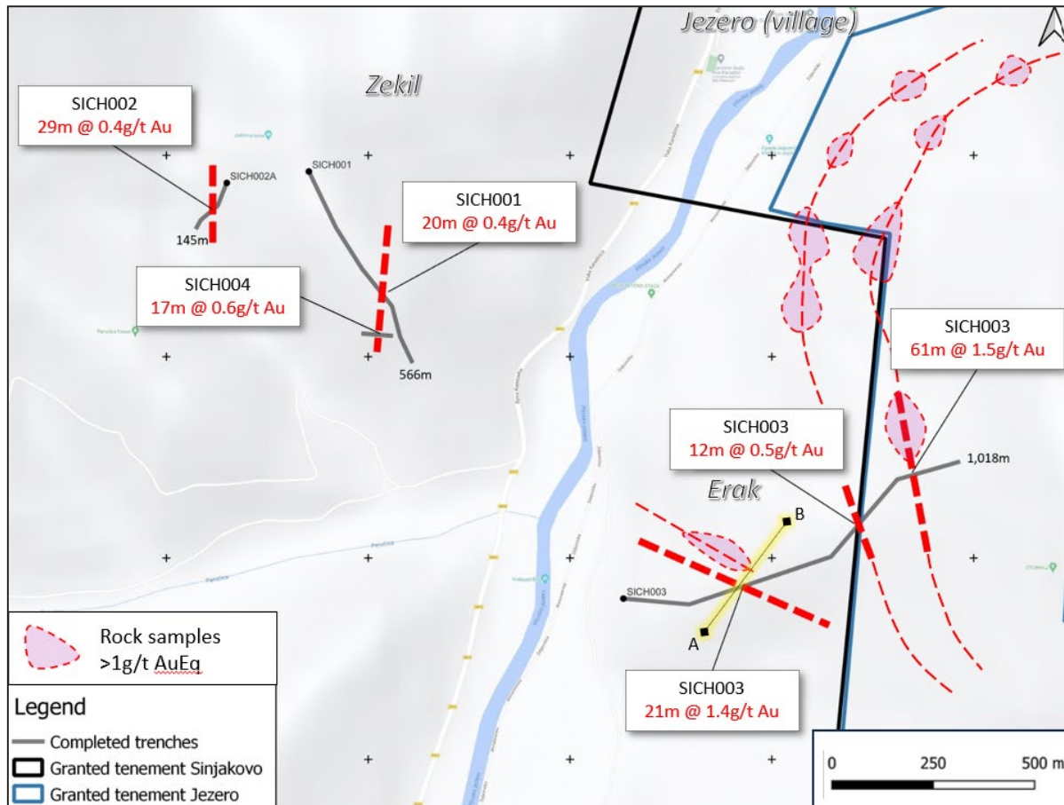
Figure 1: Plan map showing trenching results at Sinjakovo Project.
