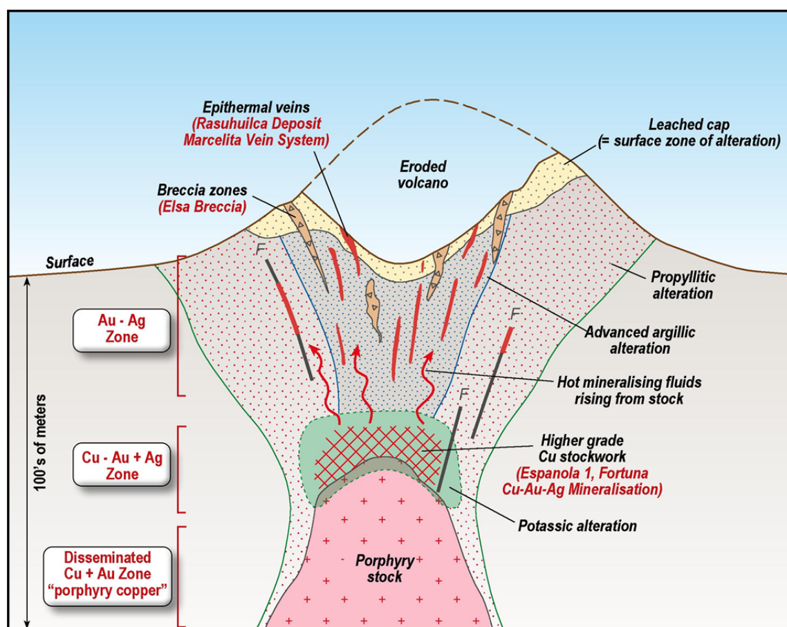
Figure 3: Schematic diagram of the Rasuhuilca porphyry exploration model, showing alteration and metal zonation. Some examples of prospects already identified are shown.
