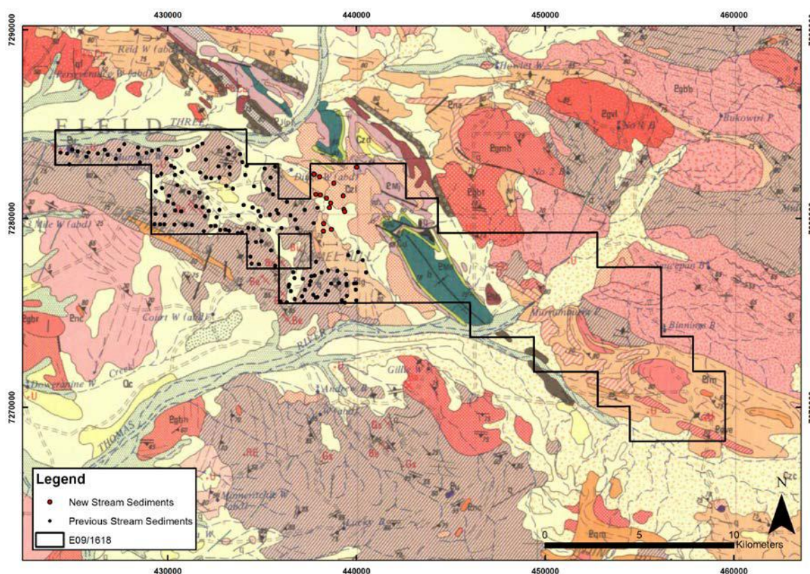
Figure 2. Sample locations on 250k Geology within tenement E09/1618. Anomalous sample locations at Camel Hill highlighted in red. (source: Arrow Minerals Ltd 'Gascoyne Lithium – E09/1618 Update April 2017' to Zeus Resources Ltd)
