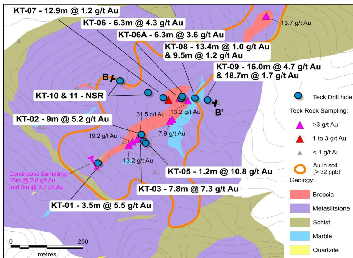
Figure 2: Kavaklitepe Kuzezy Zone Drill Hole Locations, Gold Intersections and Location of Cross Sections (B-B')
