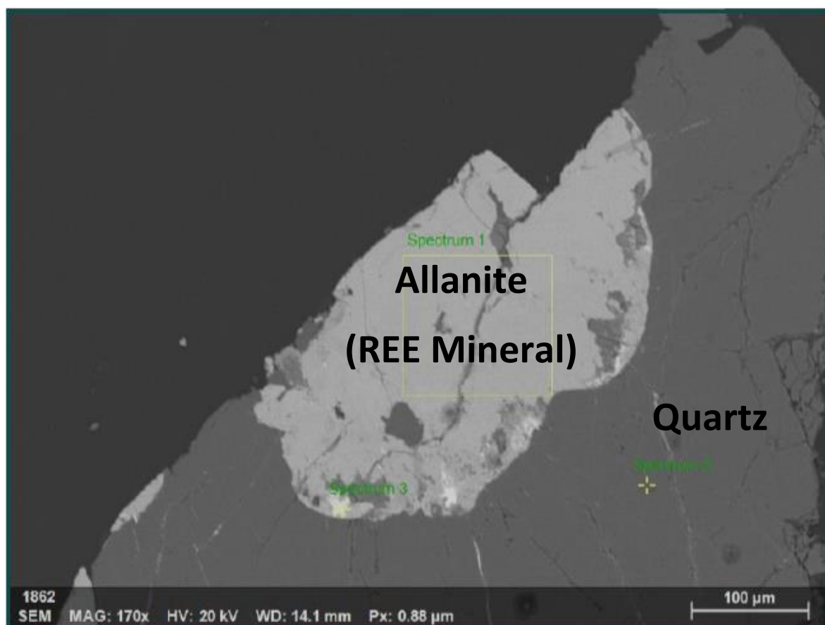
Photomicrograph of the Rare Earth Mineral Allanite Taken Under Scanning Electron Microscope (allanite grain size is approx. 0.3mm across)
