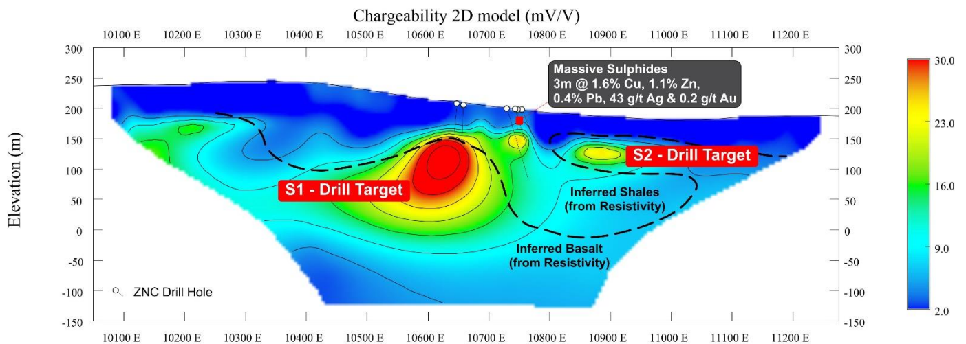
Figure 4: Snook Prospect IP Pseudosection L20,100N Showing Existing Shallow RC & DD Holes that do not reach the S1 Drill Target
