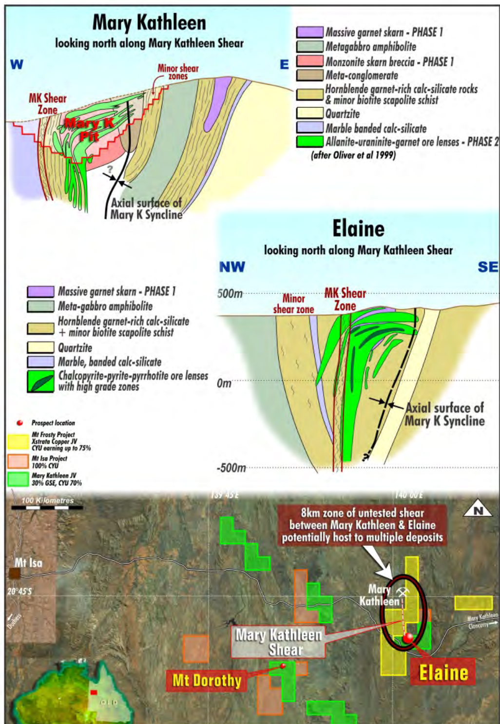
Figure 1: Mary Kathleen and Elaine comparative exploration model. The model is interpreted to be fed from a deep seated steep dipping feeder zone that has used the shear zone as a conduit, extending from depth upwards and then along and replacing the horizontal bedding of the host banded calc-silicate rocks, forming a shallow dipping to horizontal zone coming to within 50 metres of surface.
