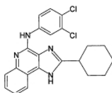
1H-imidazo[4,5-c]quinolin-4-amine Derivatives
