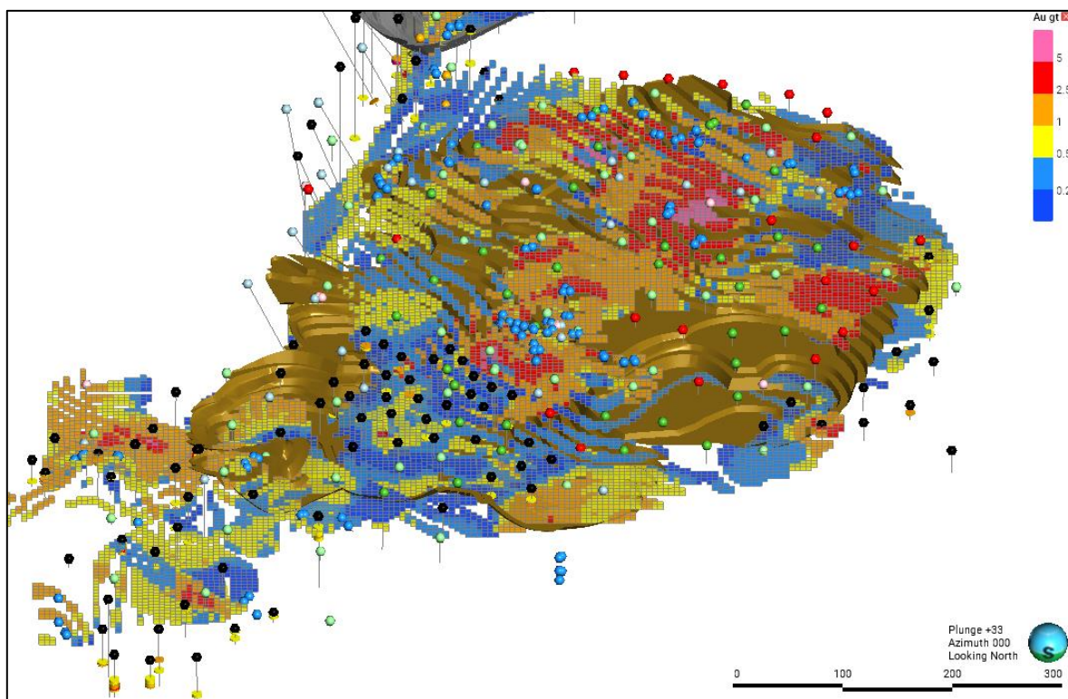
Figure 3: 3D view of Tavşan Main and South Zone showing 2025 drilling within and around the currently planned pits. The March 2024 block model is shown, coloured on the same scale as the assay results. Parts of the Main Zone have been mined already, as can be seen by blocks sitting above the topography (gold colour). Drilling and assays are only shown for 2025 for simplicity and only intercepts greater than 0.5g/t Au are shown.
