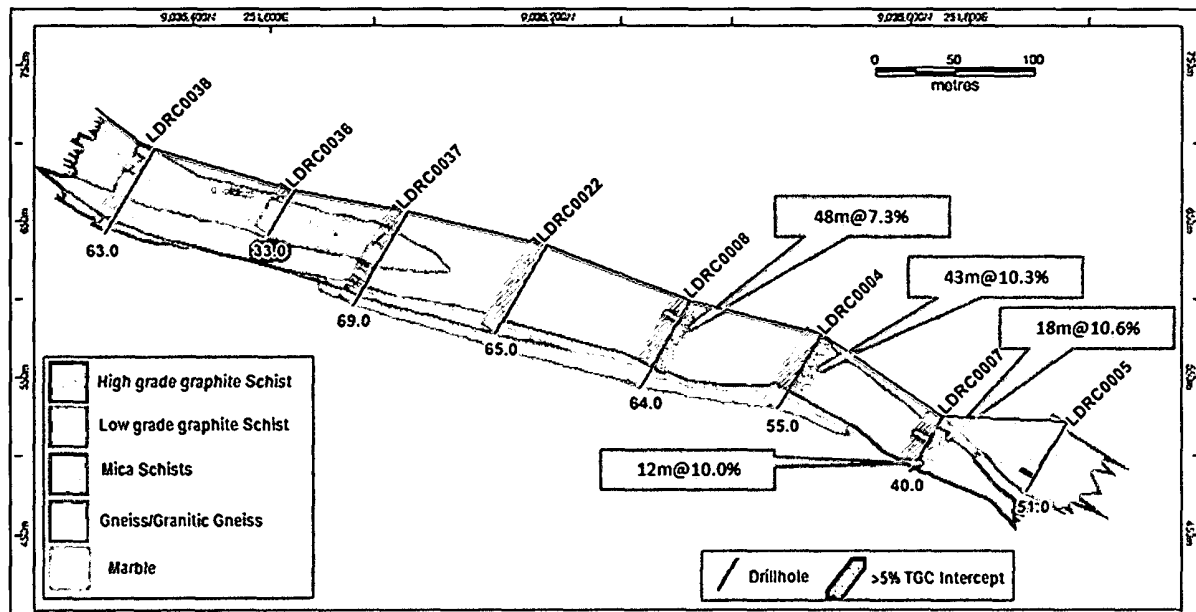
Typical Mahenge Liandu cross section showing mineralised units
