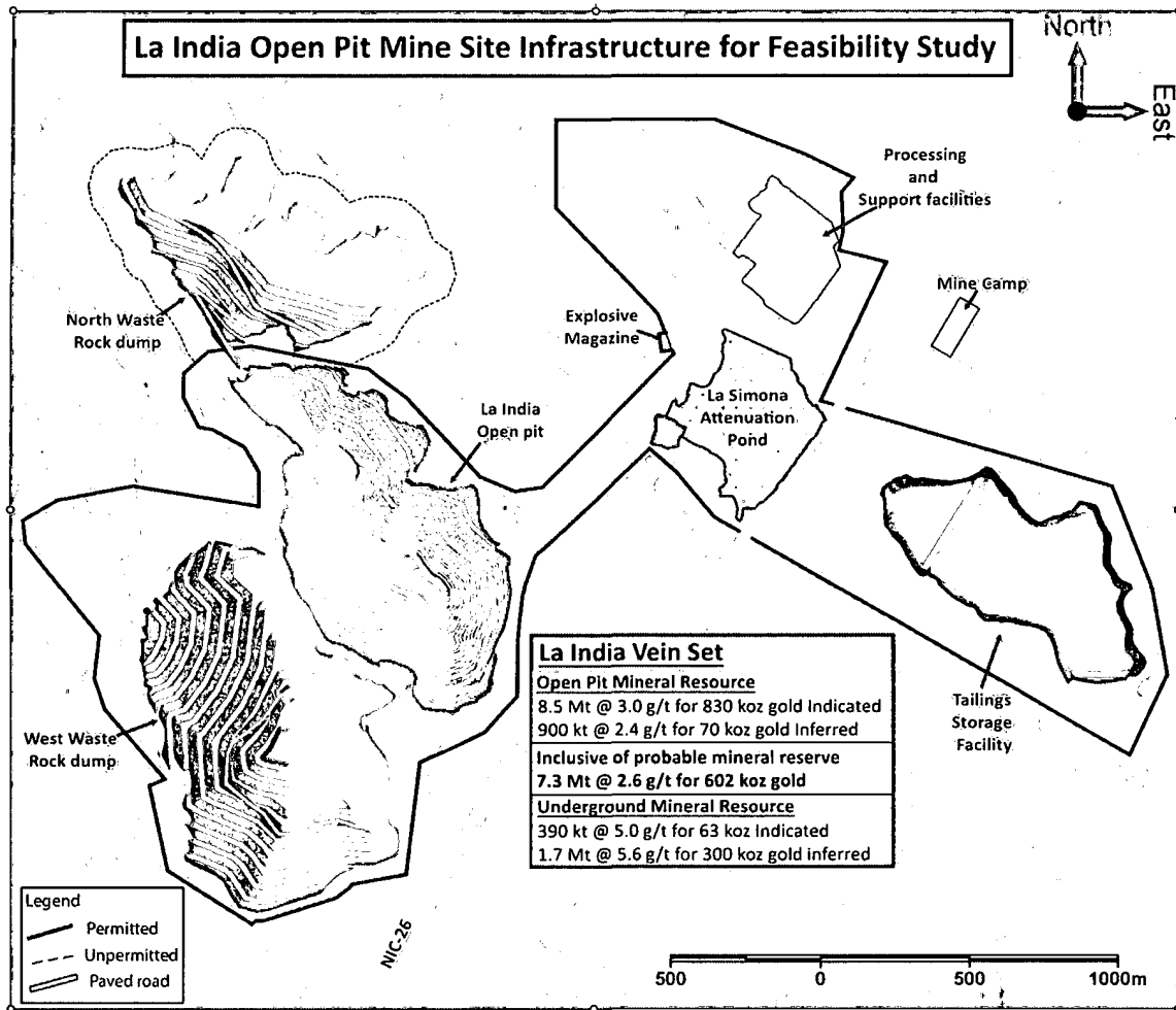
Figure 5: Site General Arrangement and Infrastructure
