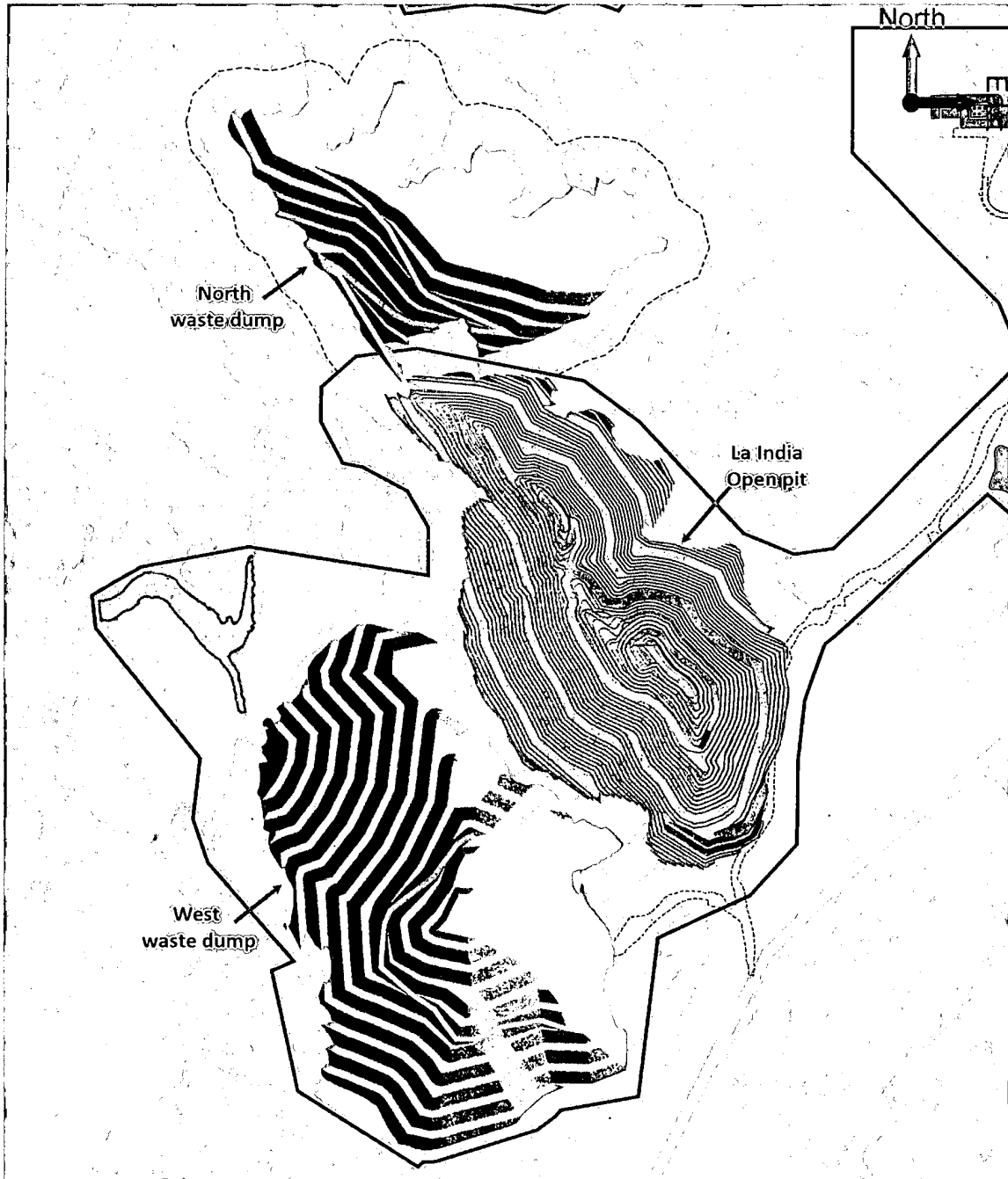
Figure 3: Ultimate Pit Design with Waste Dumps
