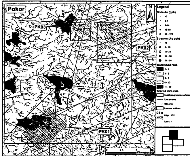
Figure 5. Soil sampling results to date at Pokor, on stream sediment geochemistry (point data and ranked watersheds)
