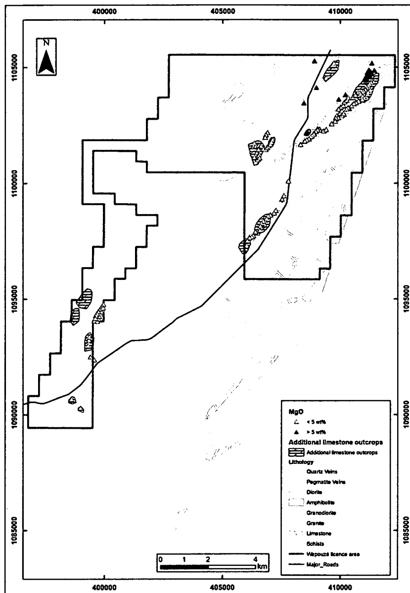
Figure 6. MgO (wt%) data for all limestone rock chip samples collected to date at Wapouzé, where CaO content is greater than 50%. Samples with <5wt% MgO and >50% CaO are considered to have appropriate carbonate content for use in the cement industry
