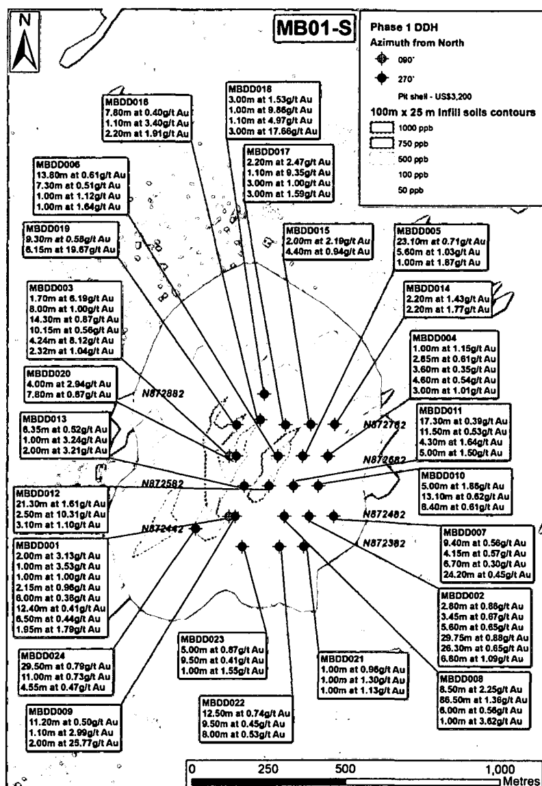
Figure 4. Phase 1 drilling plan for MB01-S with a selection of best results to date from fire assay analysis.
