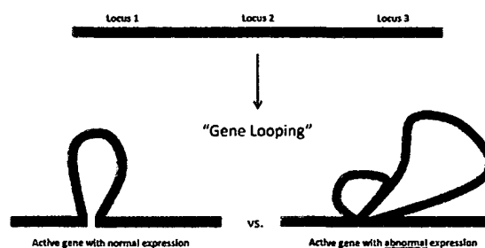
FIGURE 3 Chromosome conformations
