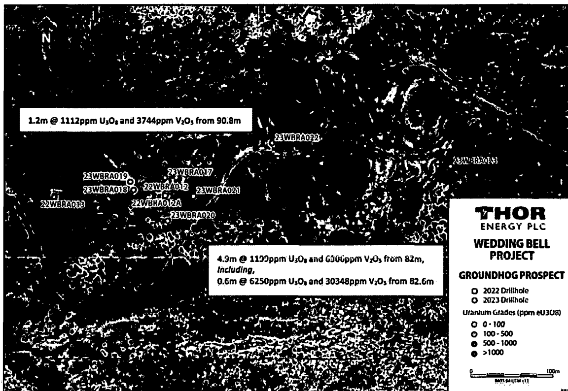
▲ Figure 6: Groundhog collar location plan showing uranium grade distribution
