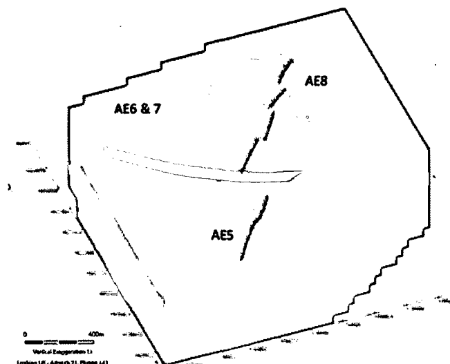
△ Figure 13: Alford East 3D ANT and Structural Model highlighting the NNE trending fault zone (red) commonly associated with copper oxide mineralisation as seen at prospect AE5 to AE8
