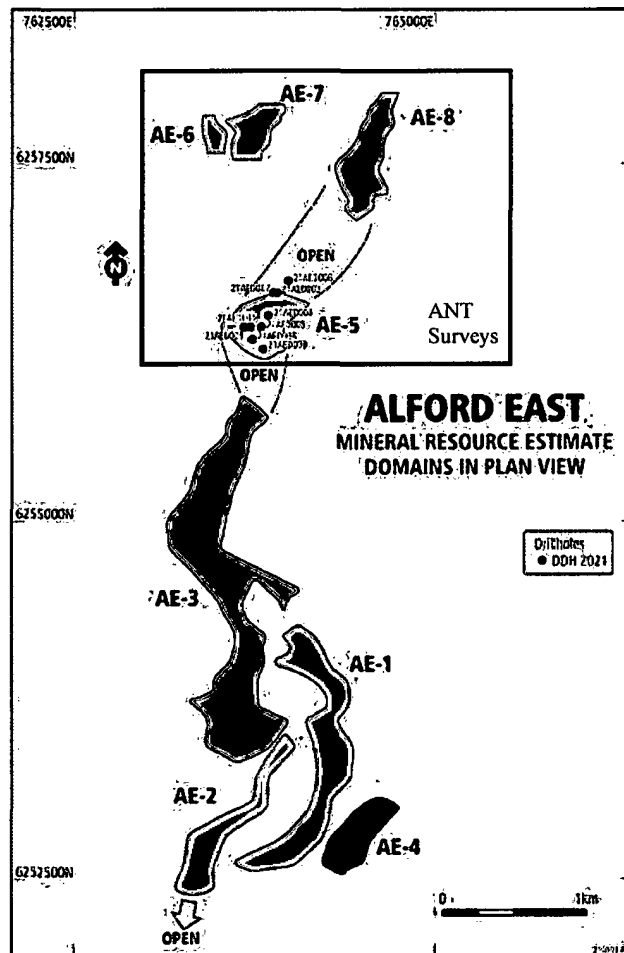
▲ Figure 11: MRE Mineralisation Domains showing ANT survey coverage
