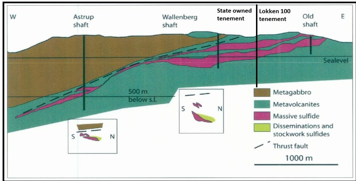
Figure 4: Løkken mine long-section showing tenement boundary (after Grenne et al 1980)
